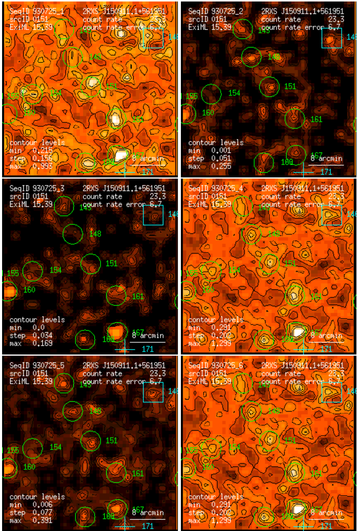
Figure 151: RASS 930725: detection 0151: band rate images, Gaussian filter: (1) PSPC channels 11 – 41, (2) 52 – 90, (3) 91 – 201, (4) 11 – 235, (5) 52 – 201, (6) 11 – 201. Broad band rates in counts/ks. Band rate contour levels in counts/ks/arcmin 2 .
