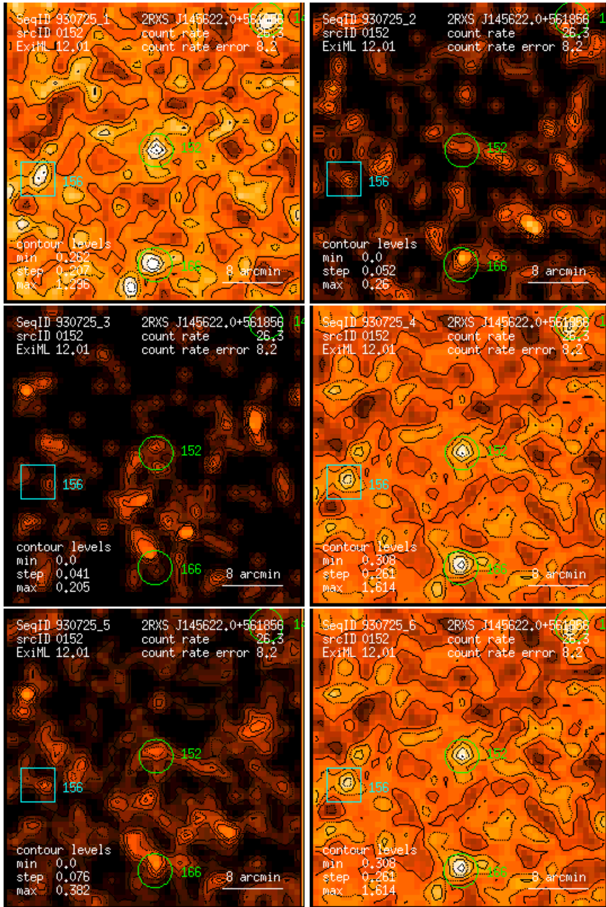
Figure 152: RASS 930725: detection 0152: band rate images, Gaussian filter: (1) PSPC channels 11 – 41, (2) 52 – 90, (3) 91 – 201, (4) 11 – 235, (5) 52 – 201, (6) 11 – 201. Broad band rates in counts/ks. Band rate contour levels in counts/ks/arcmin 2 .
