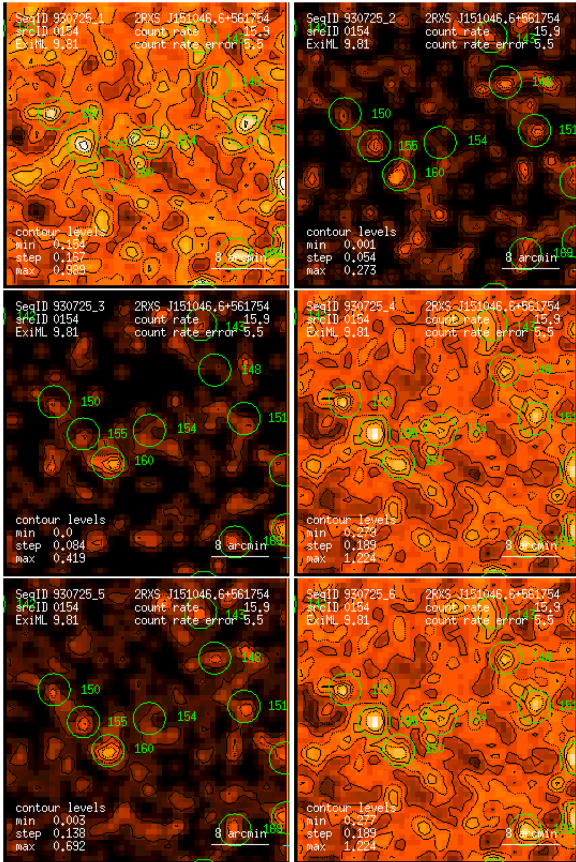
Figure 154: RASS 930725: detection 0154: band rate images, Gaussian filter: (1) PSPC channels 11 – 41, (2) 52 – 90, (3) 91 – 201, (4) 11 – 235, (5) 52 – 201, (6) 11 – 201. Broad band rates in counts/ks. Band rate contour levels in counts/ks/arcmin 2 .
