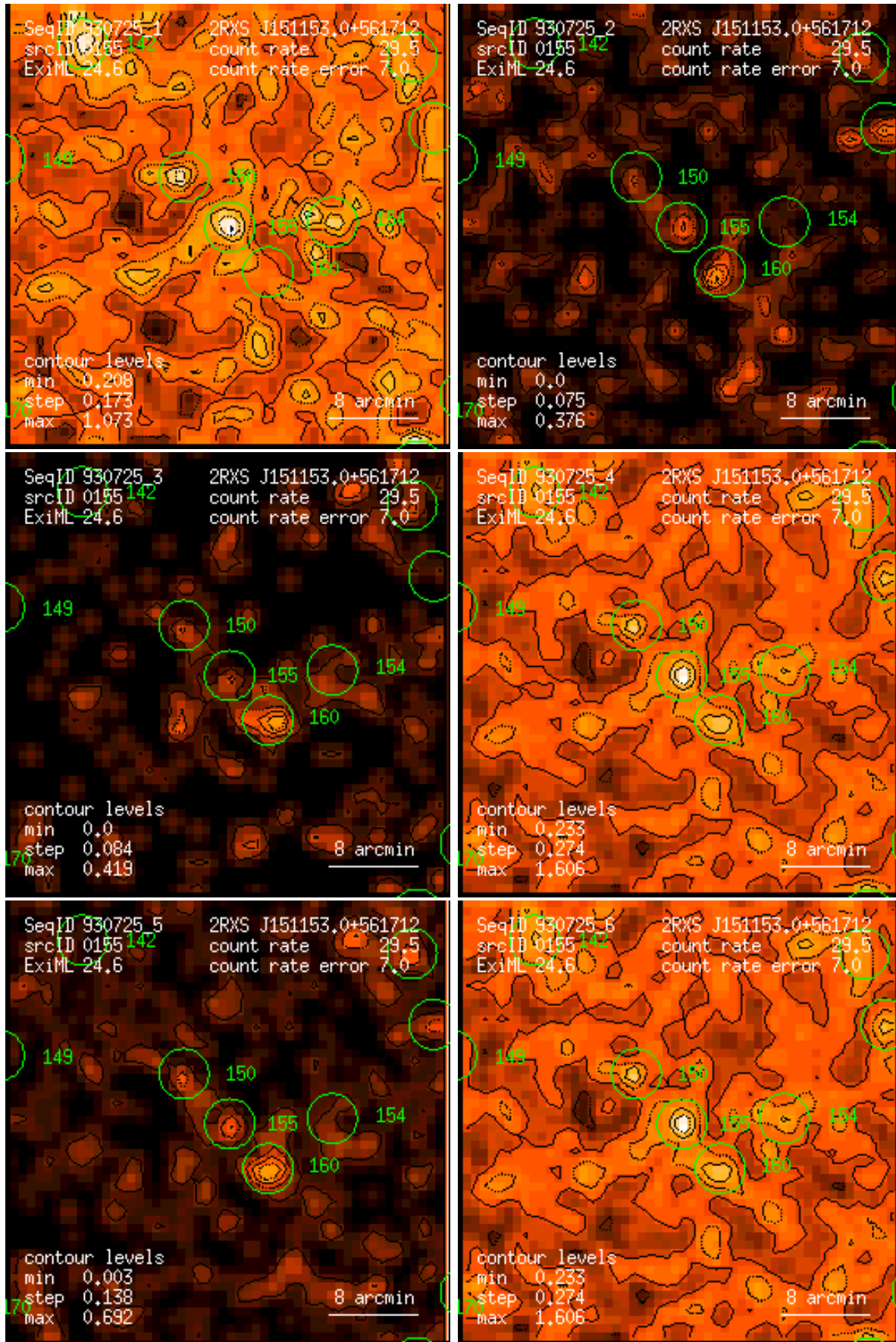
Figure 155: RASS 930725: detection 0155: band rate images, Gaussian filter: (1) PSPC channels 11 – 41, (2) 52 – 90, (3) 91 – 201, (4) 11 – 235, (5) 52 – 201, (6) 11 – 201. Broad band rates in counts/ks. Band rate contour levels in counts/ks/arcmin 2 .
