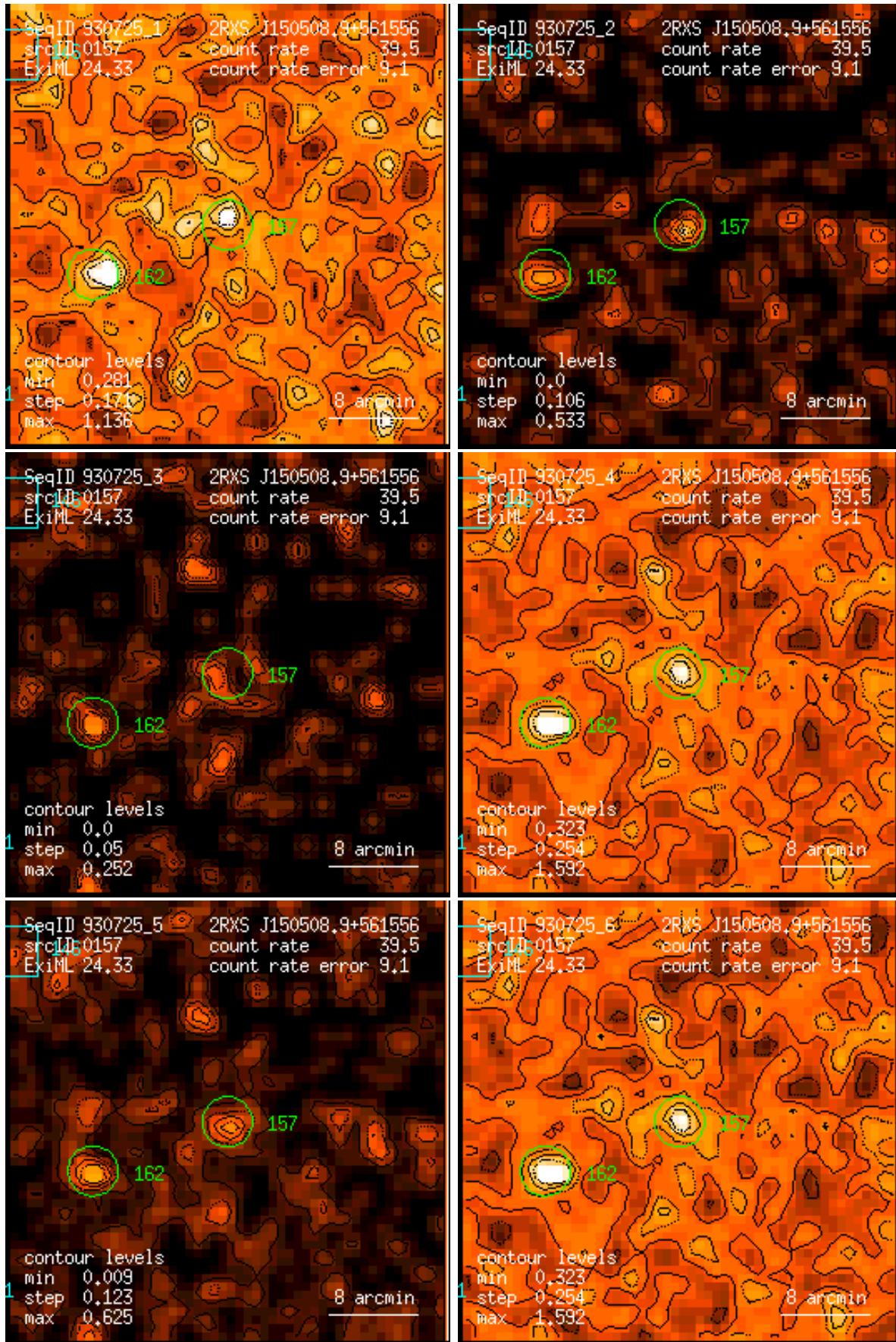
Figure 157: RASS 930725: detection 0157: band rate images, Gaussian filter: (1) PSPC channels 11 – 41, (2) 52 – 90, (3) 91 – 201, (4) 11 – 235, (5) 52 – 201, (6) 11 – 201. Broad band rates in counts/ks. Band rate contour levels in counts/ks/arcmin 2 .
