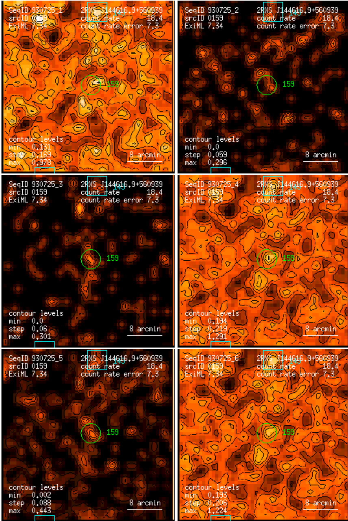
Figure 159: RASS 930725: detection 0159: band rate images, Gaussian filter: (1) PSPC channels 11 – 41, (2) 52 – 90, (3) 91 – 201, (4) 11 – 235, (5) 52 – 201, (6) 11 – 201. Broad band rates in counts/ks. Band rate contour levels in counts/ks/arcmin 2 .
