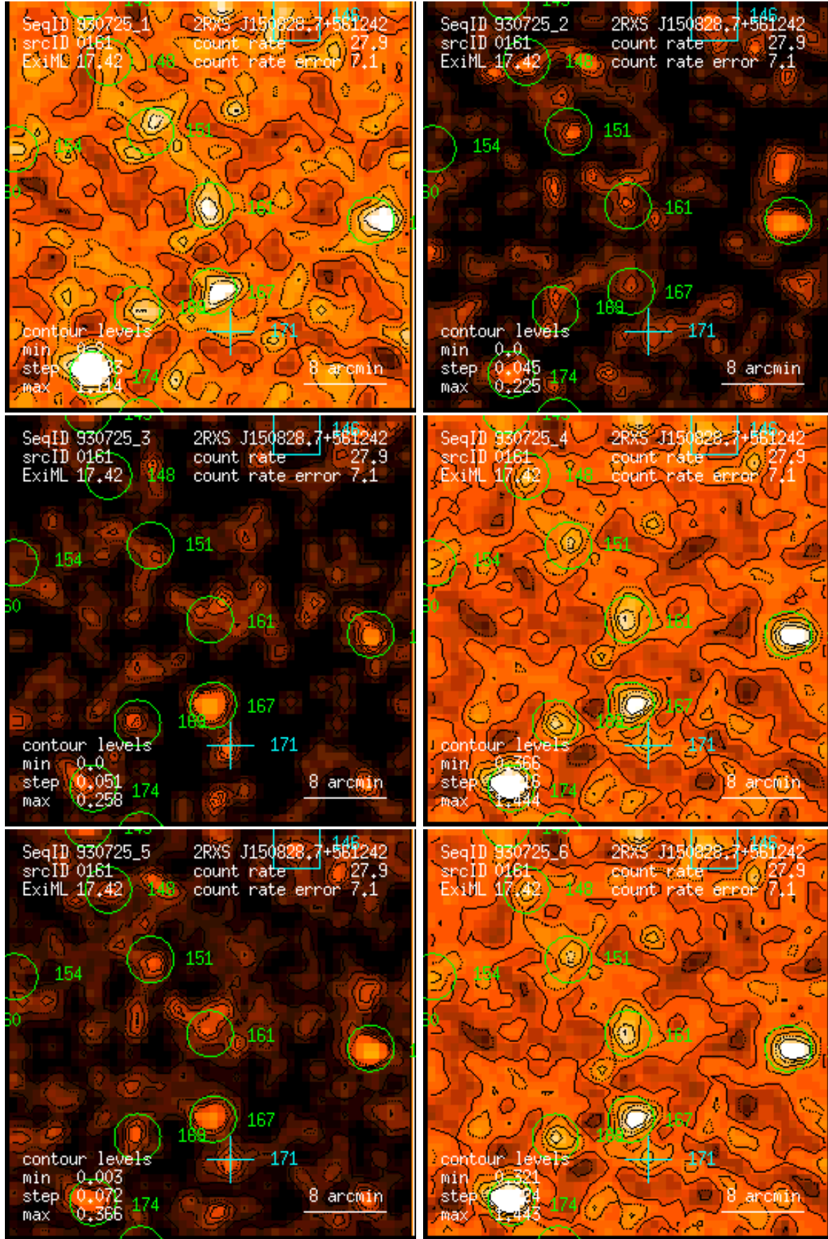
Figure 161: RASS 930725: detection 0161: band rate images, Gaussian filter: (1) PSPC channels 11 – 41, (2) 52 – 90, (3) 91 – 201, (4) 11 – 235, (5) 52 – 201, (6) 11 – 201. Broad band rates in counts/ks. Band rate contour levels in counts/ks/arcmin 2 .
