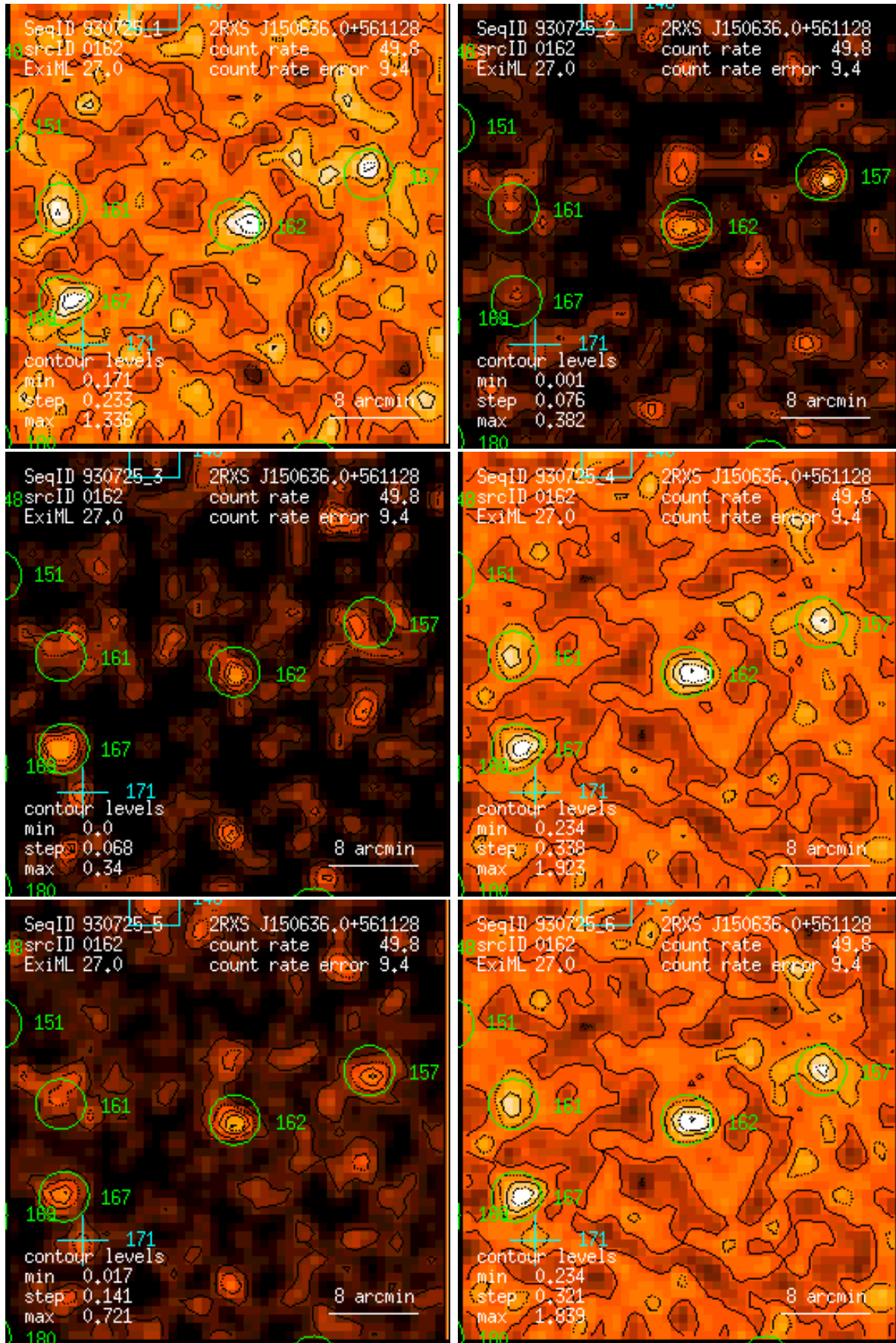
Figure 162: RASS 930725: detection 0162: band rate images, Gaussian filter: (1) PSPC channels 11 – 41, (2) 52 – 90, (3) 91 – 201, (4) 11 – 235, (5) 52 – 201, (6) 11 – 201. Broad band rates in counts/ks. Band rate contour levels in counts/ks/arcmin 2 .
