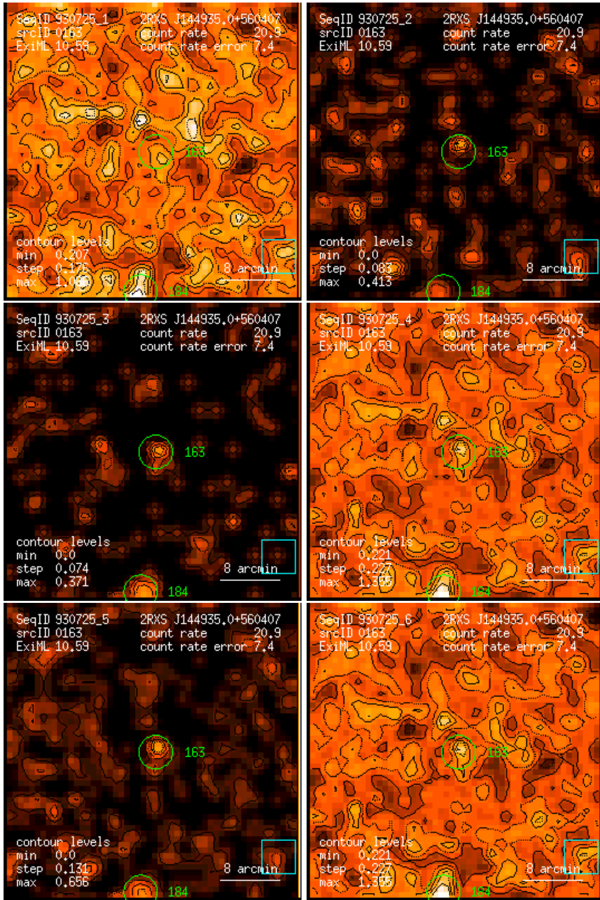
Figure 163: RASS 930725: detection 0163: band rate images, Gaussian filter: (1) PSPC channels 11 – 41, (2) 52 – 90, (3) 91 – 201, (4) 11 – 235, (5) 52 – 201, (6) 11 – 201. Broad band rates in counts/ks. Band rate contour levels in counts/ks/arcmin 2 .
