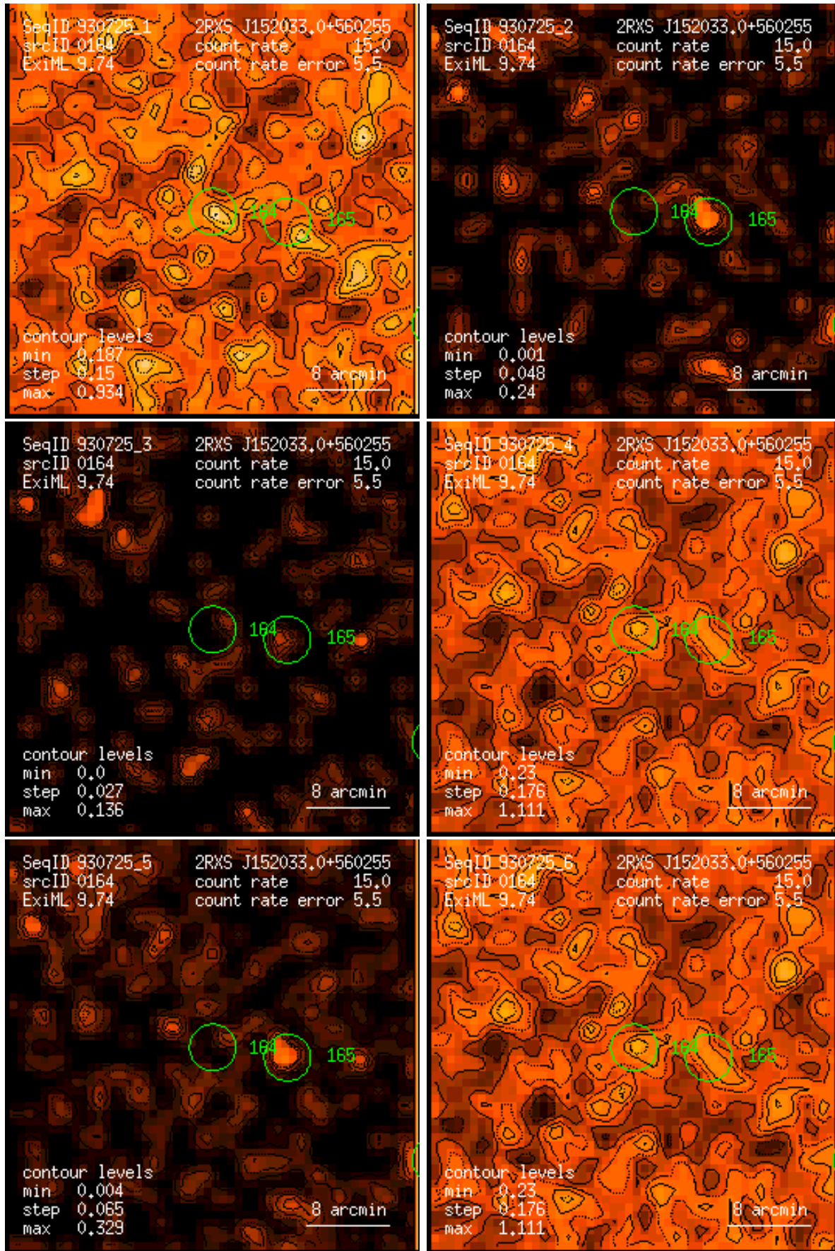
Figure 164: RASS 930725: detection 0164: band rate images, Gaussian filter: (1) PSPC channels 11 – 41, (2) 52 – 90, (3) 91 – 201, (4) 11 – 235, (5) 52 – 201, (6) 11 – 201. Broad band rates in counts/ks. Band rate contour levels in counts/ks/arcmin 2 .
