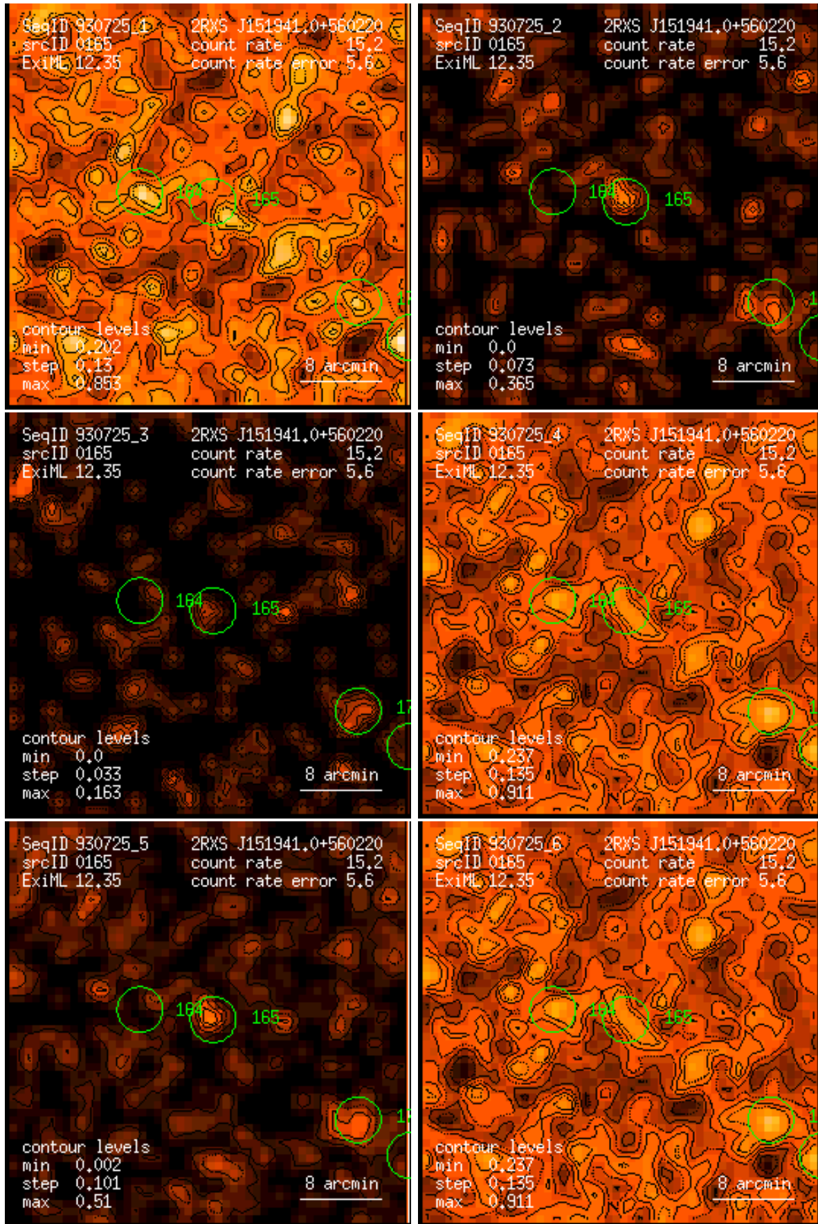
Figure 165: RASS 930725: detection 0165: band rate images, Gaussian filter: (1) PSPC channels 11 – 41, (2) 52 – 90, (3) 91 – 201, (4) 11 – 235, (5) 52 – 201, (6) 11 – 201. Broad band rates in counts/ks. Band rate contour levels in counts/ks/arcmin 2 .
