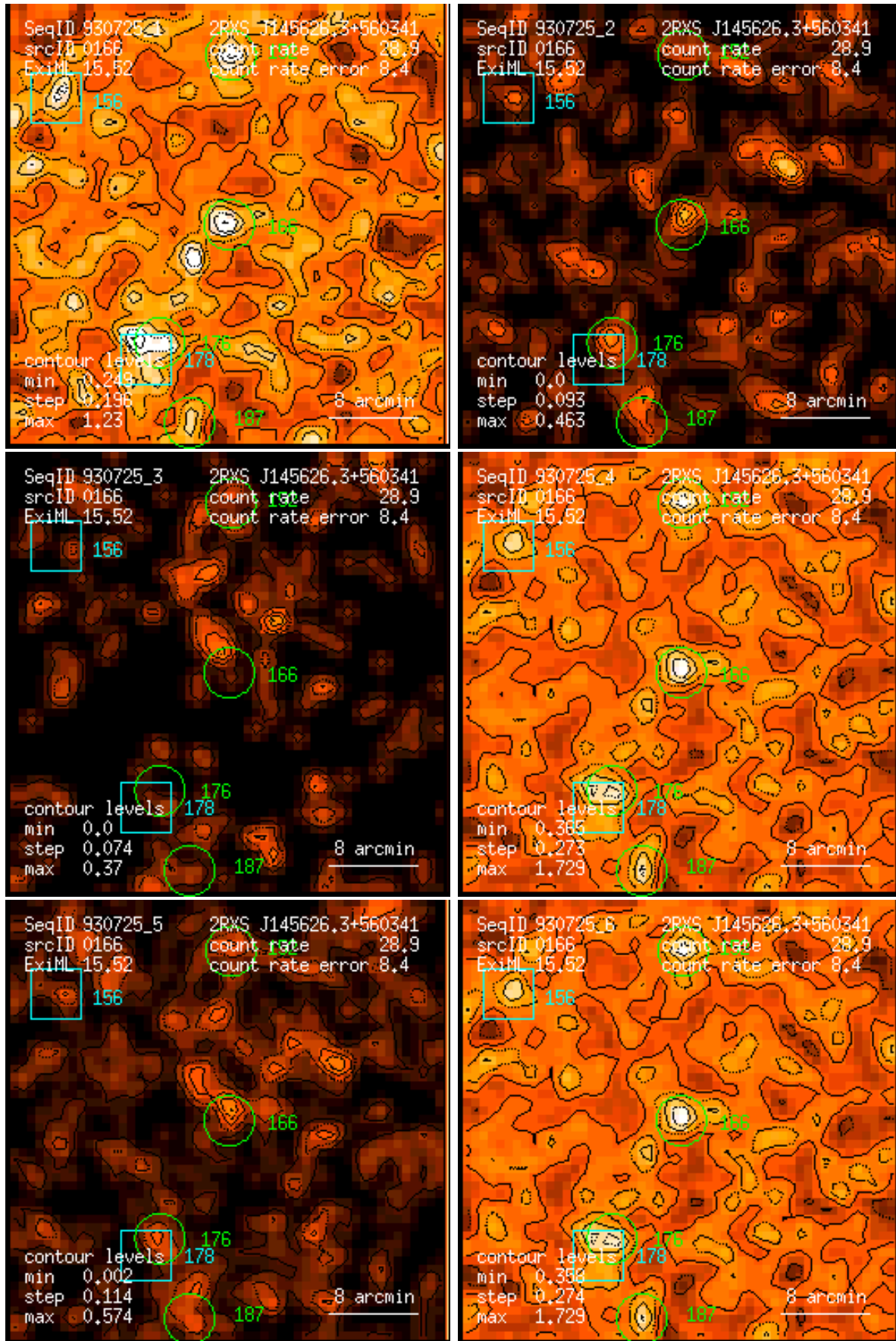
Figure 166: RASS 930725: detection 0166: band rate images, Gaussian filter: (1) PSPC channels 11 – 41, (2) 52 – 90, (3) 91 – 201, (4) 11 – 235, (5) 52 – 201, (6) 11 – 201. Broad band rates in counts/ks. Band rate contour levels in counts/ks/arcmin 2 .
