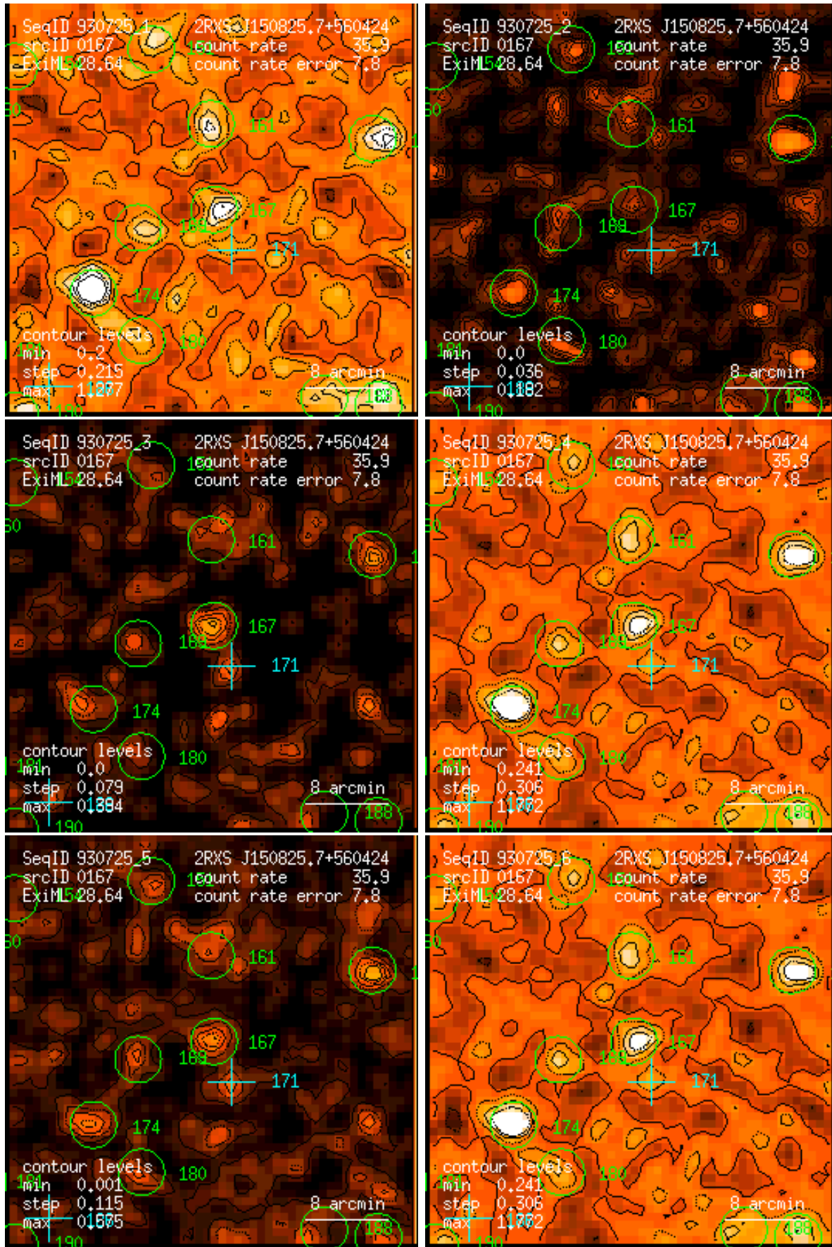
Figure 167: RASS 930725: detection 0167: band rate images, Gaussian filter: (1) PSPC channels 11 – 41, (2) 52 – 90, (3) 91 – 201, (4) 11 – 235, (5) 52 – 201, (6) 11 – 201. Broad band rates in counts/ks. Band rate contour levels in counts/ks/arcmin 2 .
