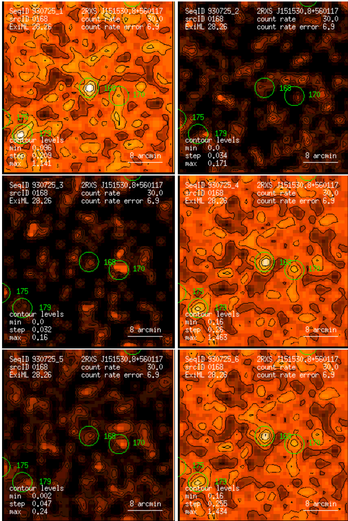
Figure 168: RASS 930725: detection 0168: band rate images, Gaussian filter: (1) PSPC channels 11 – 41, (2) 52 – 90, (3) 91 – 201, (4) 11 – 235, (5) 52 – 201, (6) 11 – 201. Broad band rates in counts/ks. Band rate contour levels in counts/ks/arcmin 2 .
