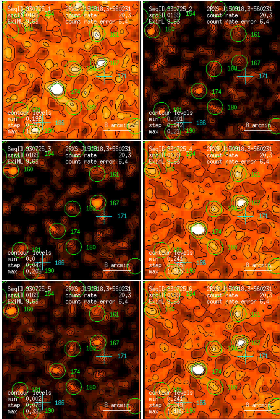
Figure 169: RASS 930725: detection 0169: band rate images, Gaussian filter: (1) PSPC channels 11 – 41, (2) 52 – 90, (3) 91 – 201, (4) 11 – 235, (5) 52 – 201, (6) 11 – 201. Broad band rates in counts/ks. Band rate contour levels in counts/ks/arcmin 2 .
