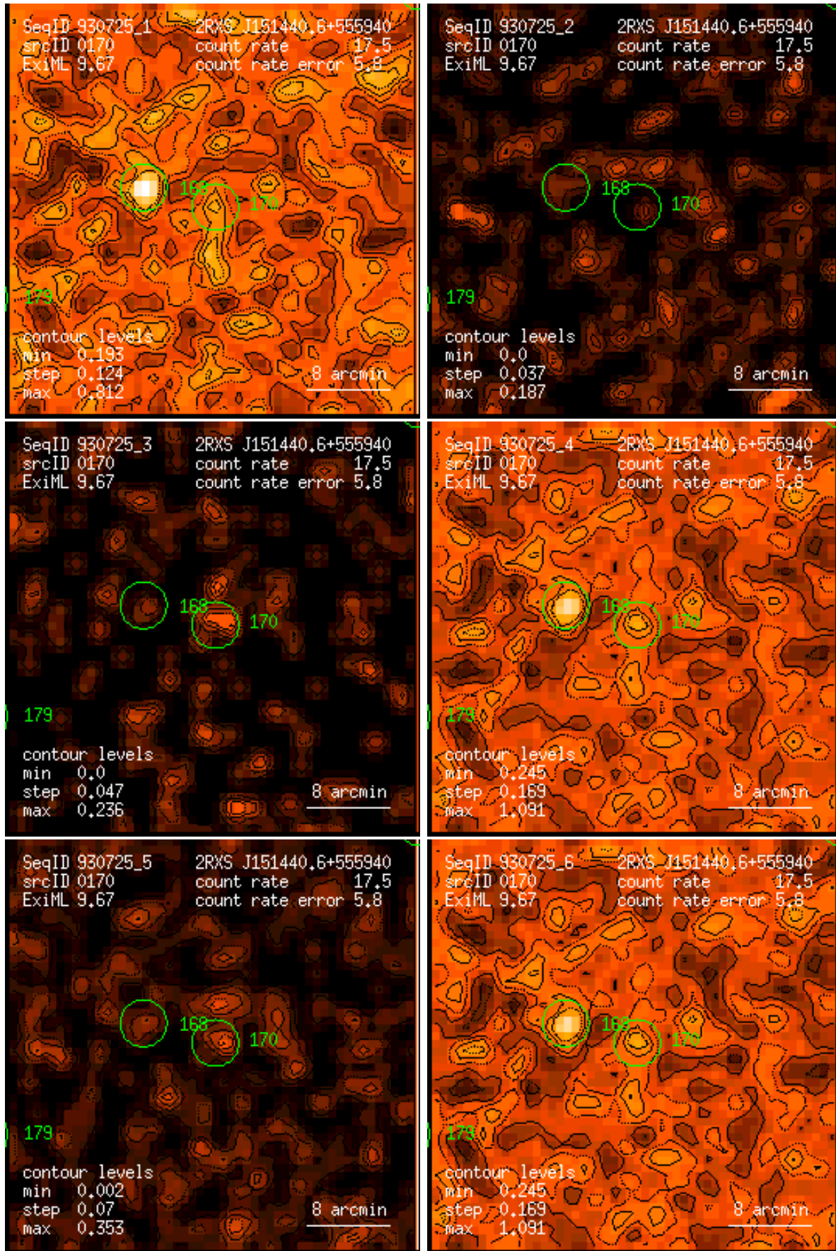
Figure 170: RASS 930725: detection 0170: band rate images, Gaussian filter: (1) PSPC channels 11 – 41, (2) 52 – 90, (3) 91 – 201, (4) 11 – 235, (5) 52 – 201, (6) 11 – 201. Broad band rates in counts/ks. Band rate contour levels in counts/ks/arcmin 2 .
