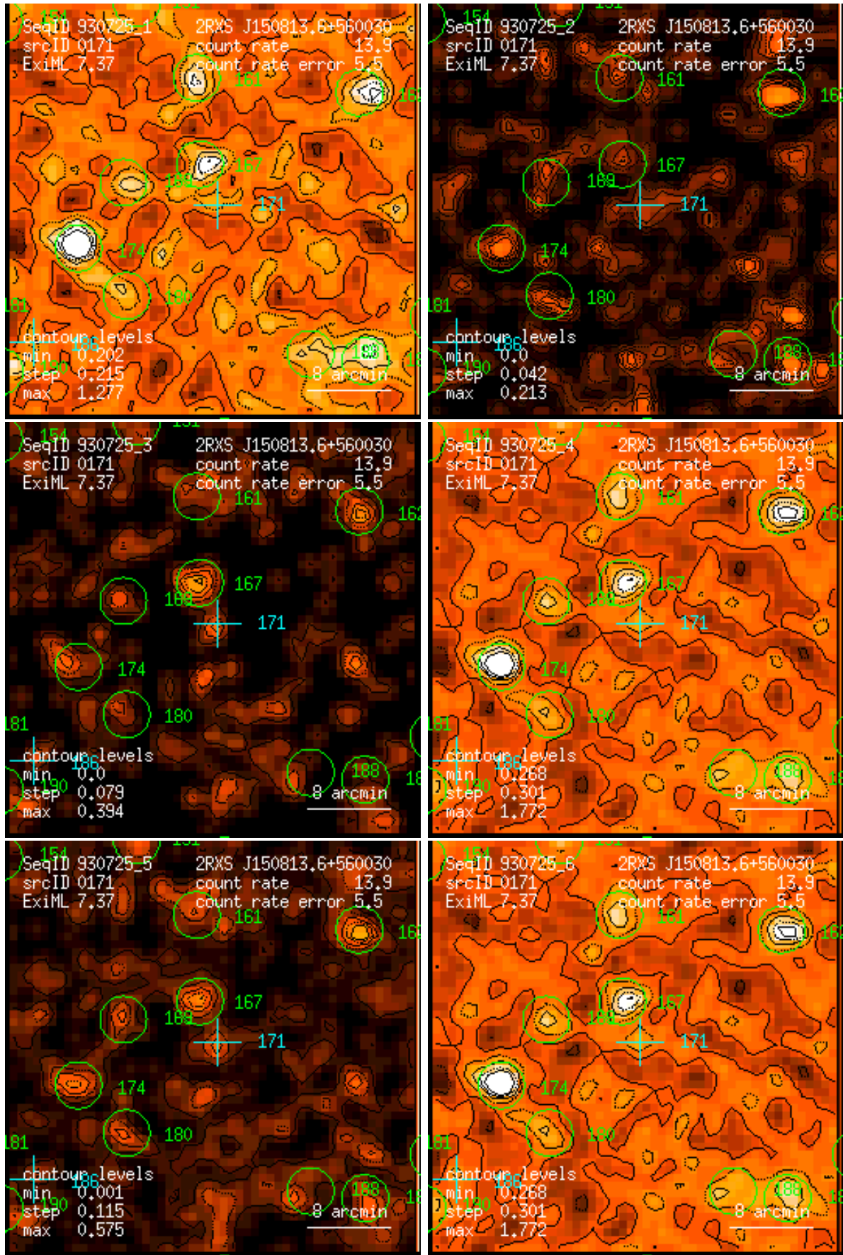
Figure 171: RASS 930725: detection 0171: band rate images, Gaussian filter: (1) PSPC channels 11 – 41, (2) 52 – 90, (3) 91 – 201, (4) 11 – 235, (5) 52 – 201, (6) 11 – 201. Broad band rates in counts/ks. Band rate contour levels in counts/ks/arcmin 2 .
