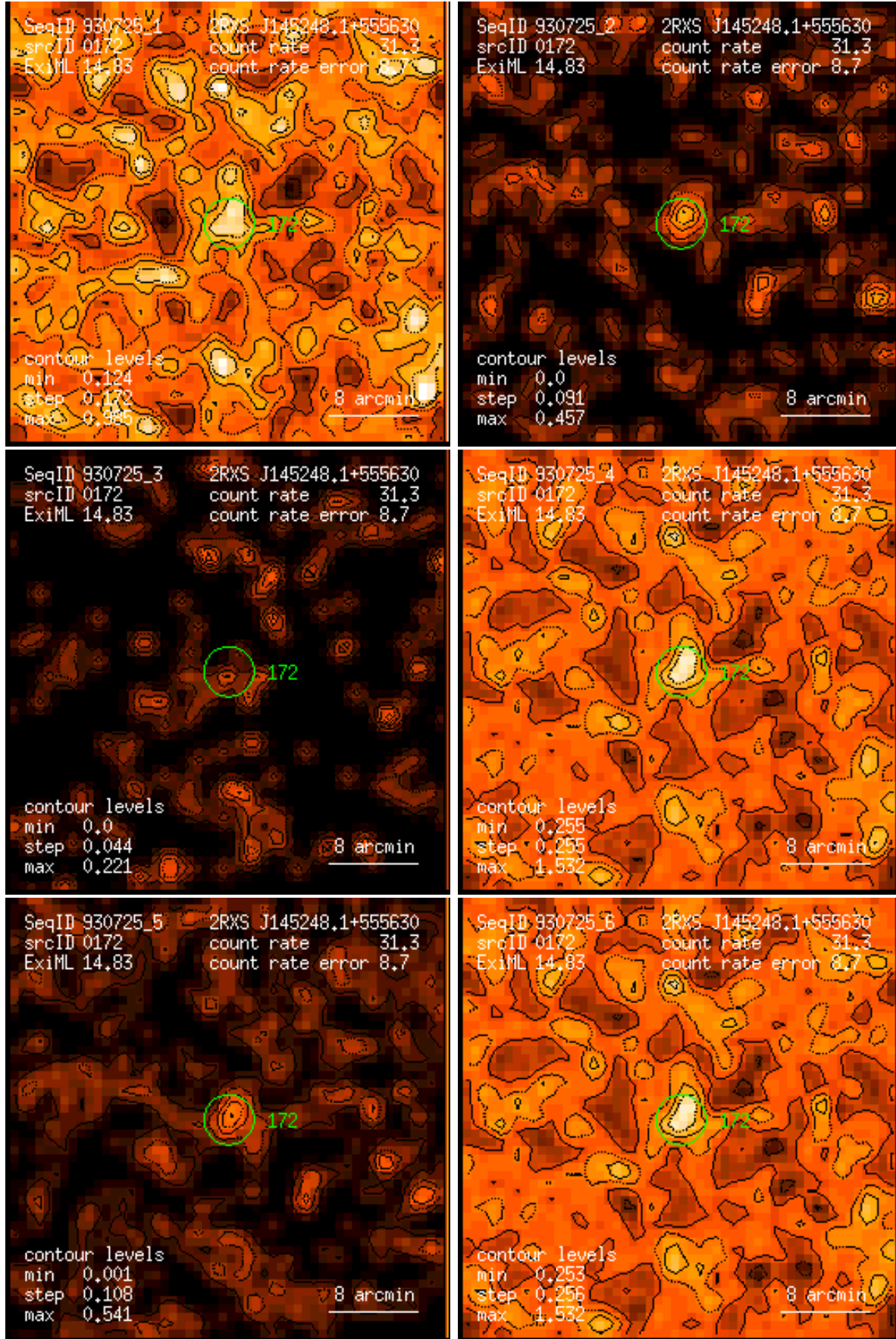
Figure 172: RASS 930725: detection 0172: band rate images, Gaussian filter: (1) PSPC channels 11 – 41, (2) 52 – 90, (3) 91 – 201, (4) 11 – 235, (5) 52 – 201, (6) 11 – 201. Broad band rates in counts/ks. Band rate contour levels in counts/ks/arcmin 2 .
