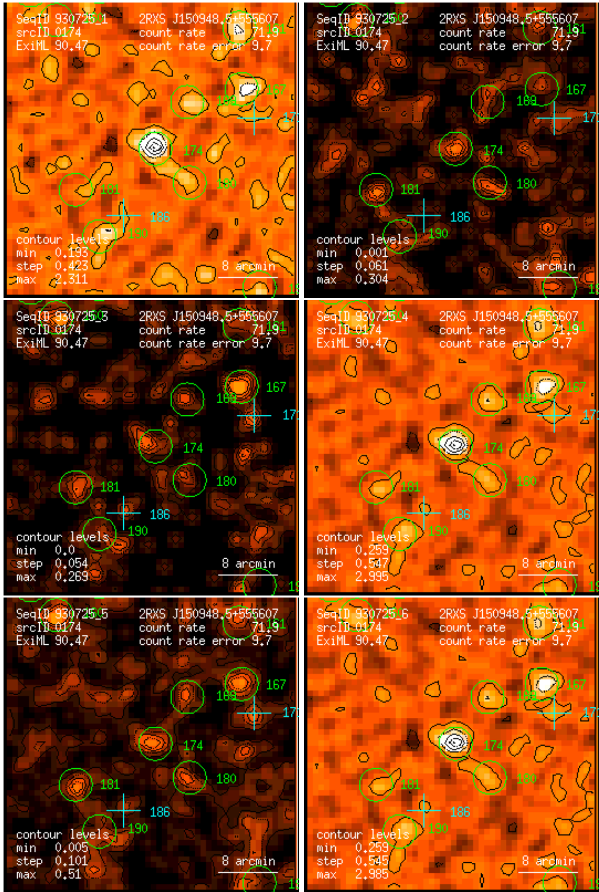
Figure 174: RASS 930725: detection 0174: band rate images, Gaussian filter: (1) PSPC channels 11 – 41, (2) 52 – 90, (3) 91 – 201, (4) 11 – 235, (5) 52 – 201, (6) 11 – 201. Broad band rates in counts/ks. Band rate contour levels in counts/ks/arcmin 2 .
