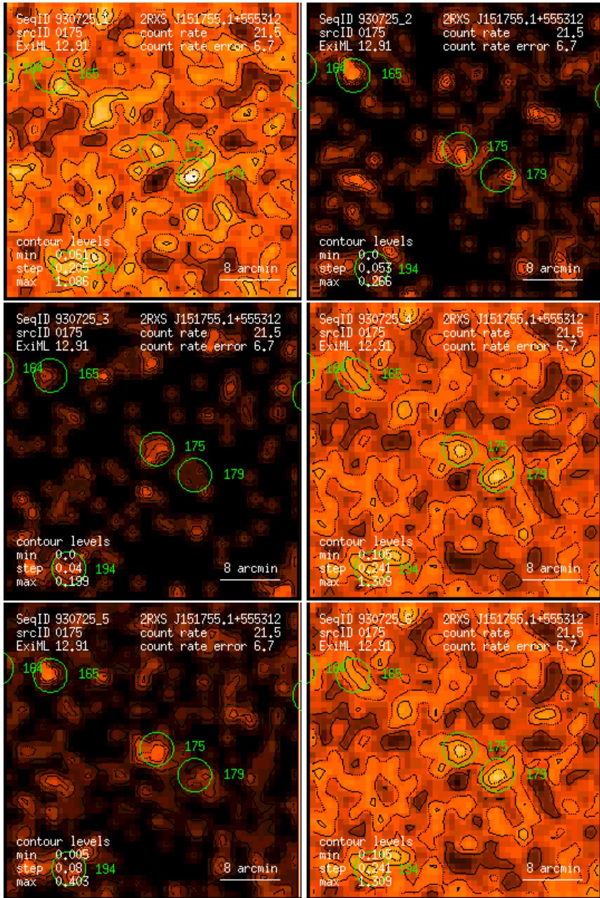
Figure 175: RASS 930725: detection 0175: band rate images, Gaussian filter: (1) PSPC channels 11 – 41, (2) 52 – 90, (3) 91 – 201, (4) 11 – 235, (5) 52 – 201, (6) 11 – 201. Broad band rates in counts/ks. Band rate contour levels in counts/ks/arcmin 2 .
