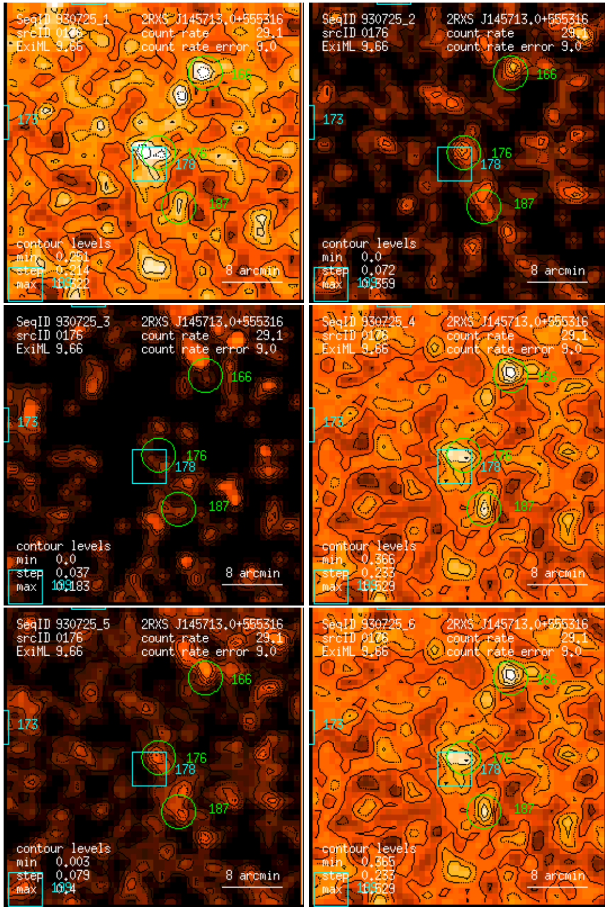
Figure 176: RASS 930725: detection 0176: band rate images, Gaussian filter: (1) PSPC channels 11 – 41, (2) 52 – 90, (3) 91 – 201, (4) 11 – 235, (5) 52 – 201, (6) 11 – 201. Broad band rates in counts/ks. Band rate contour levels in counts/ks/arcmin 2 .
