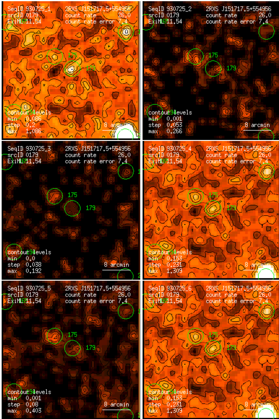
Figure 179: RASS 930725: detection 0179: band rate images, Gaussian filter: (1) PSPC channels 11 – 41, (2) 52 – 90, (3) 91 – 201, (4) 11 – 235, (5) 52 – 201, (6) 11 – 201. Broad band rates in counts/ks. Band rate contour levels in counts/ks/arcmin 2 .
