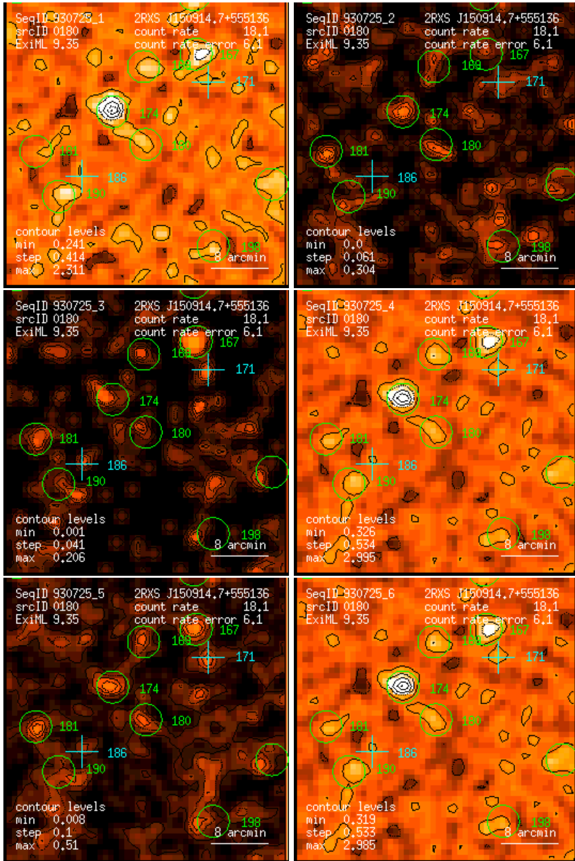
Figure 180: RASS 930725: detection 0180: band rate images, Gaussian filter: (1) PSPC channels 11 – 41, (2) 52 – 90, (3) 91 – 201, (4) 11 – 235, (5) 52 – 201, (6) 11 – 201. Broad band rates in counts/ks. Band rate contour levels in counts/ks/arcmin 2 .
