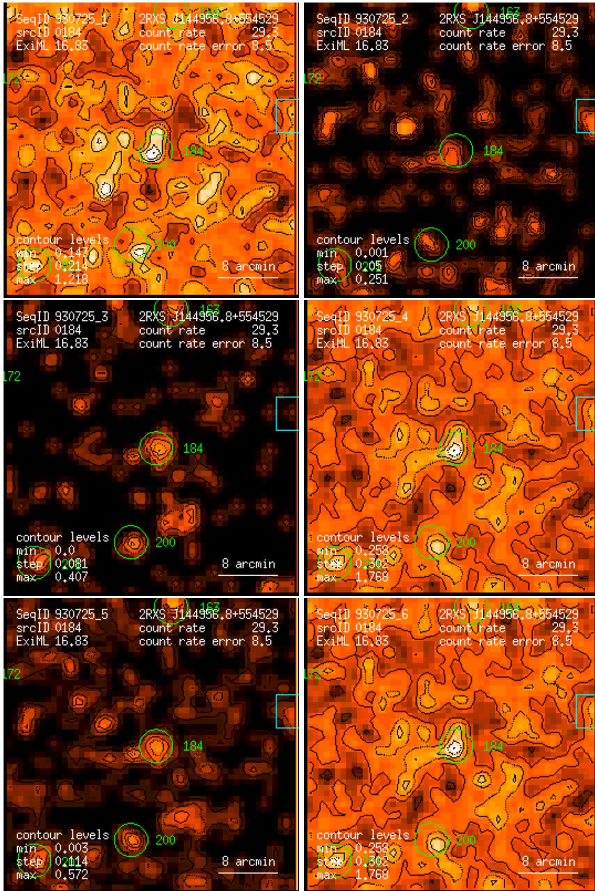
Figure 184: RASS 930725: detection 0184: band rate images, Gaussian filter: (1) PSPC channels 11 – 41, (2) 52 – 90, (3) 91 – 201, (4) 11 – 235, (5) 52 – 201, (6) 11 – 201. Broad band rates in counts/ks. Band rate contour levels in counts/ks/arcmin 2 .
