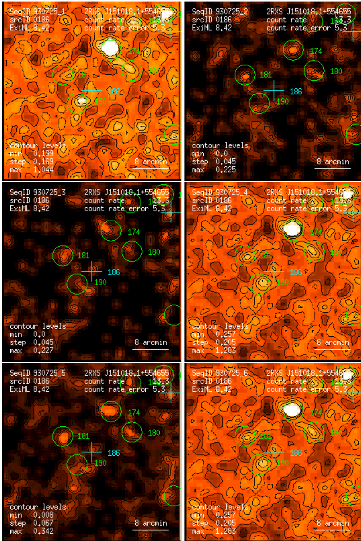
Figure 186: RASS 930725: detection 0186: band rate images, Gaussian filter: (1) PSPC channels 11 – 41, (2) 52 – 90, (3) 91 – 201, (4) 11 – 235, (5) 52 – 201, (6) 11 – 201. Broad band rates in counts/ks. Band rate contour levels in counts/ks/arcmin 2 .
