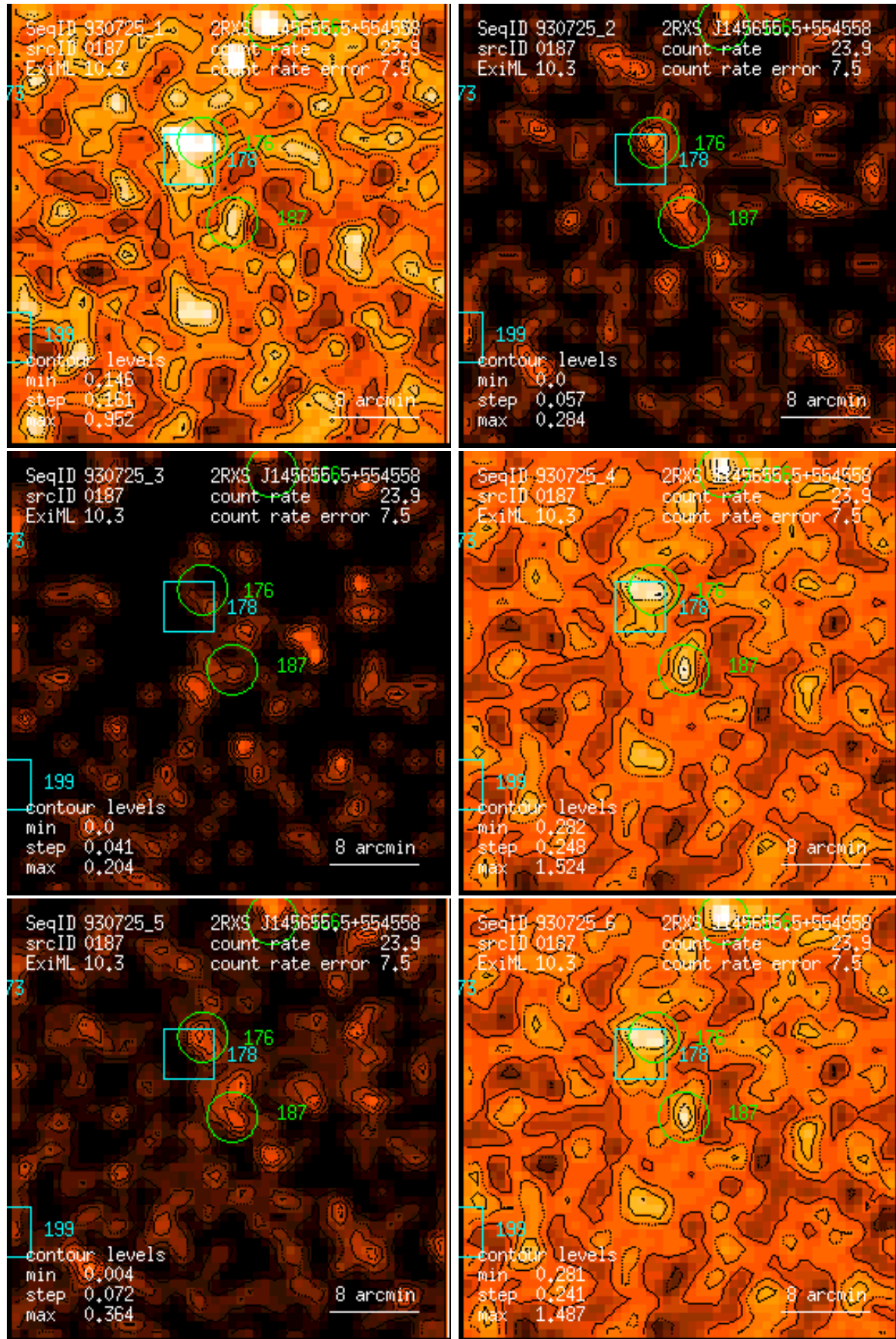
Figure 187: RASS 930725: detection 0187: band rate images, Gaussian filter: (1) PSPC channels 11 – 41, (2) 52 – 90, (3) 91 – 201, (4) 11 – 235, (5) 52 – 201, (6) 11 – 201. Broad band rates in counts/ks. Band rate contour levels in counts/ks/arcmin 2 .
