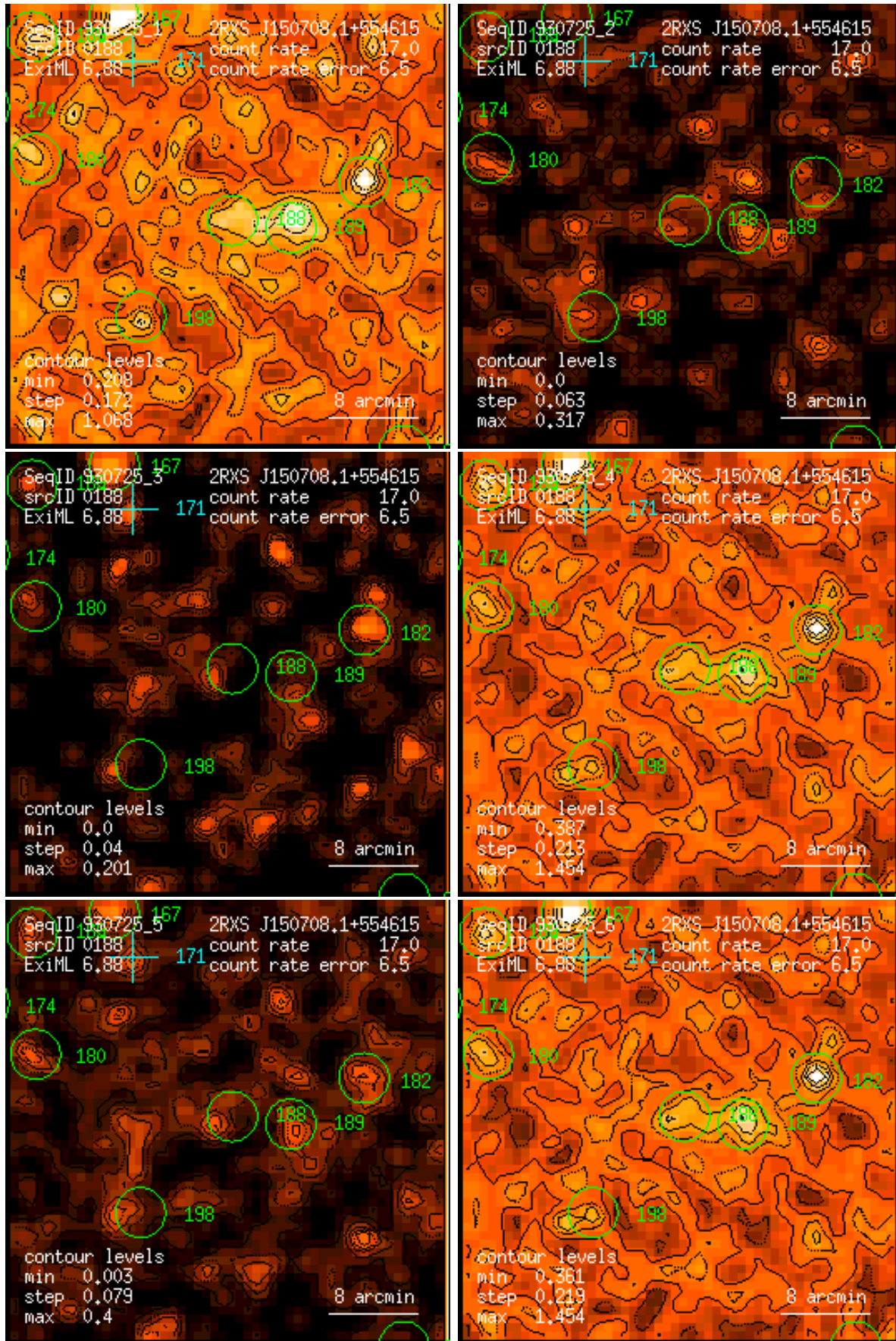
Figure 188: RASS 930725: detection 0188: band rate images, Gaussian filter: (1) PSPC channels 11 – 41, (2) 52 – 90, (3) 91 – 201, (4) 11 – 235, (5) 52 – 201, (6) 11 – 201. Broad band rates in counts/ks. Band rate contour levels in counts/ks/arcmin 2 .
