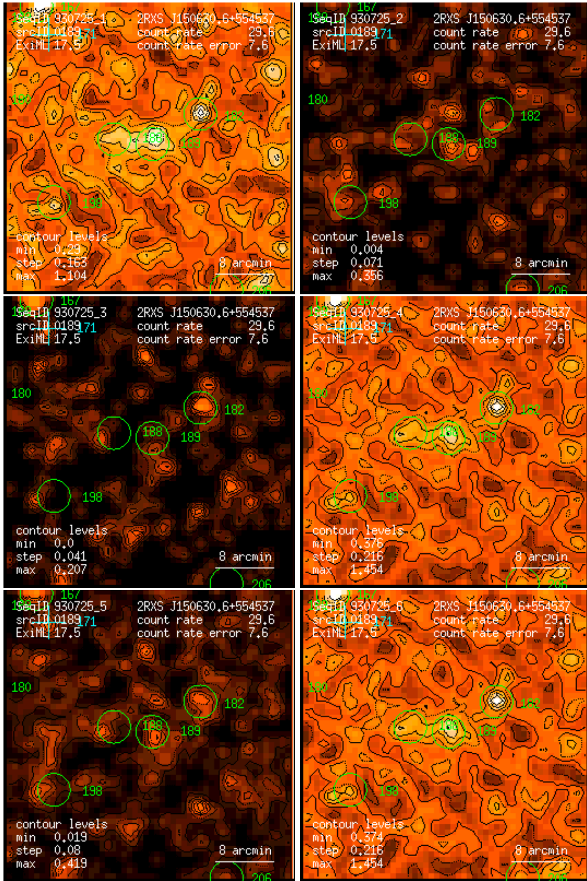
Figure 189: RASS 930725: detection 0189: band rate images, Gaussian filter: (1) PSPC channels 11 – 41, (2) 52 – 90, (3) 91 – 201, (4) 11 – 235, (5) 52 – 201, (6) 11 – 201. Broad band rates in counts/ks. Band rate contour levels in counts/ks/arcmin 2 .
