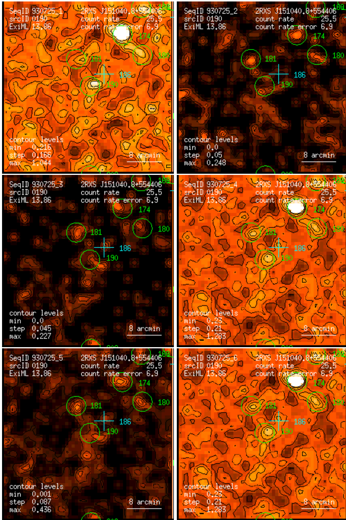
Figure 190: RASS 930725: detection 0190: band rate images, Gaussian filter: (1) PSPC channels 11 – 41, (2) 52 – 90, (3) 91 – 201, (4) 11 – 235, (5) 52 – 201, (6) 11 – 201. Broad band rates in counts/ks. Band rate contour levels in counts/ks/arcmin 2 .
