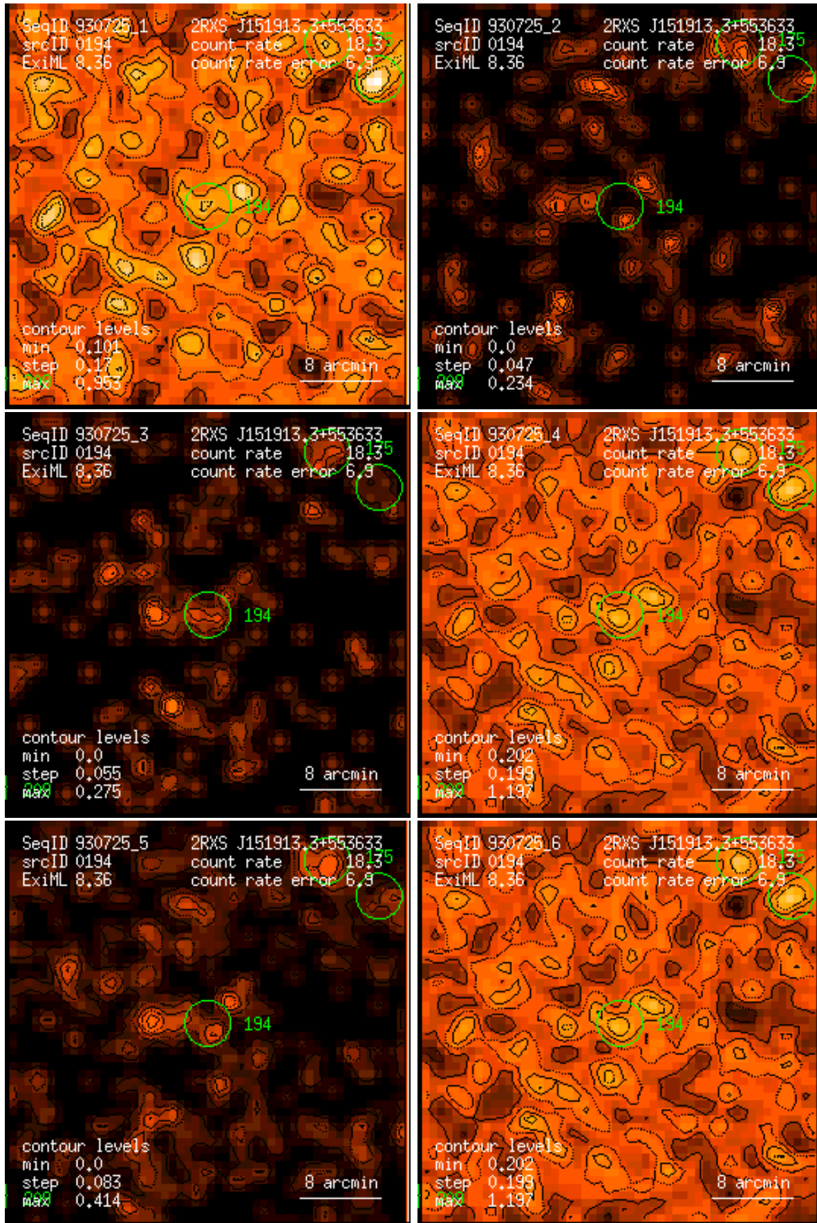
Figure 194: RASS 930725: detection 0194: band rate images, Gaussian filter: (1) PSPC channels 11 – 41, (2) 52 – 90, (3) 91 – 201, (4) 11 – 235, (5) 52 – 201, (6) 11 – 201. Broad band rates in counts/ks. Band rate contour levels in counts/ks/arcmin 2 .
