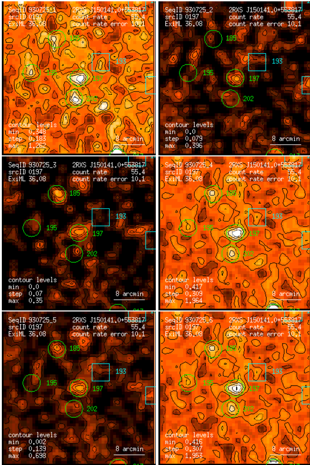
Figure 197: RASS 930725: detection 0197: band rate images, Gaussian filter: (1) PSPC channels 11 – 41, (2) 52 – 90, (3) 91 – 201, (4) 11 – 235, (5) 52 – 201, (6) 11 – 201. Broad band rates in counts/ks. Band rate contour levels in counts/ks/arcmin 2 .
