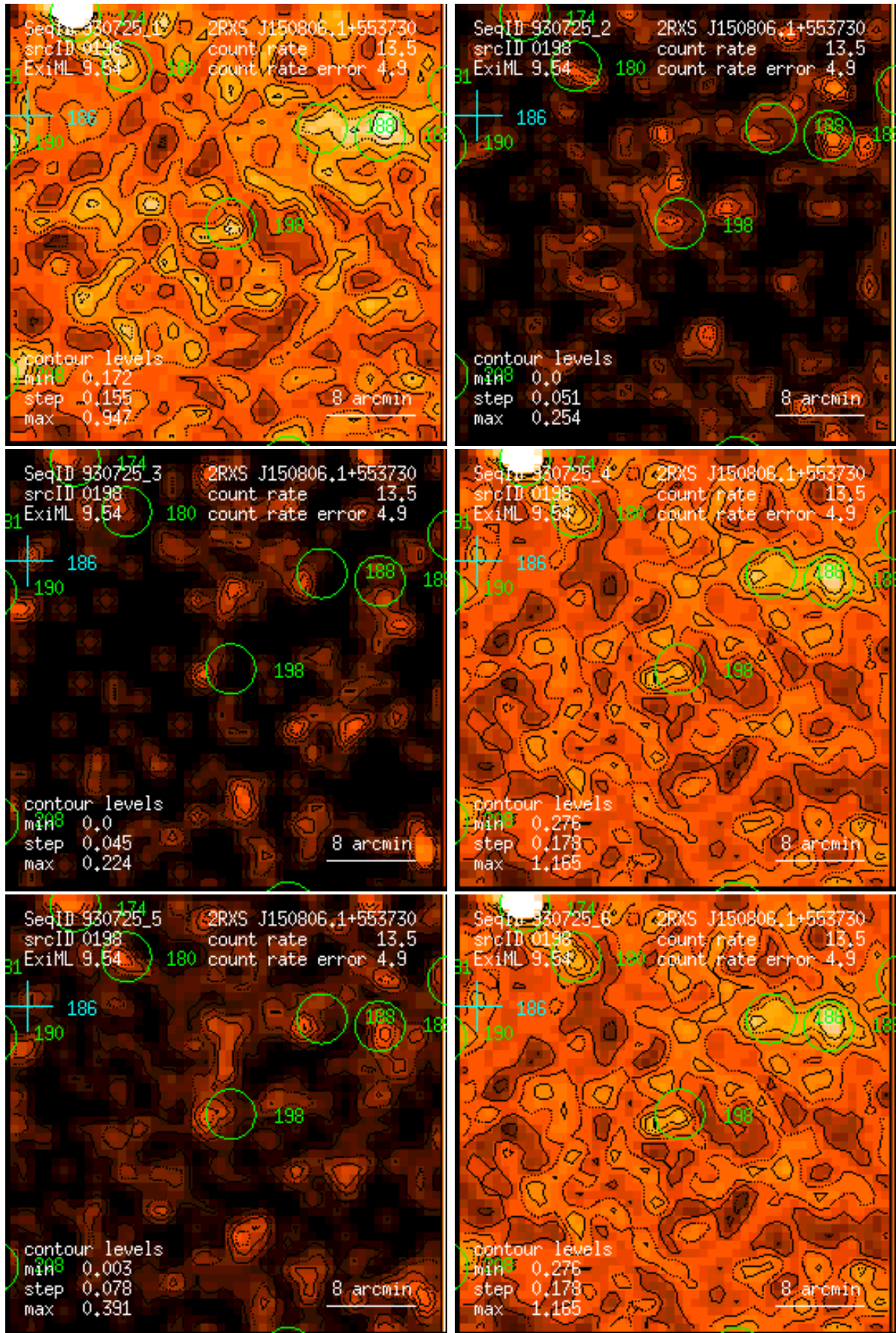
Figure 198: RASS 930725: detection 0198: band rate images, Gaussian filter: (1) PSPC channels 11 – 41, (2) 52 – 90, (3) 91 – 201, (4) 11 – 235, (5) 52 – 201, (6) 11 – 201. Broad band rates in counts/ks. Band rate contour levels in counts/ks/arcmin 2 .
