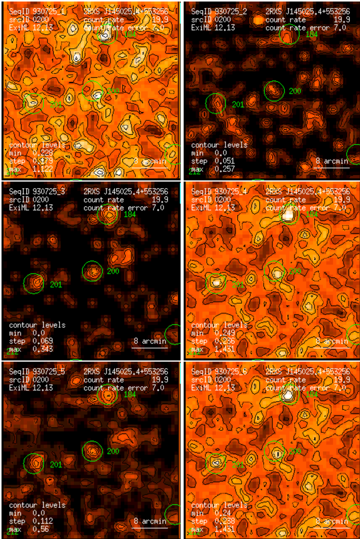
Figure 200: RASS 930725: detection 0200: band rate images, Gaussian filter: (1) PSPC channels 11 – 41, (2) 52 – 90, (3) 91 – 201, (4) 11 – 235, (5) 52 – 201, (6) 11 – 201. Broad band rates in counts/ks. Band rate contour levels in counts/ks/arcmin 2 .
