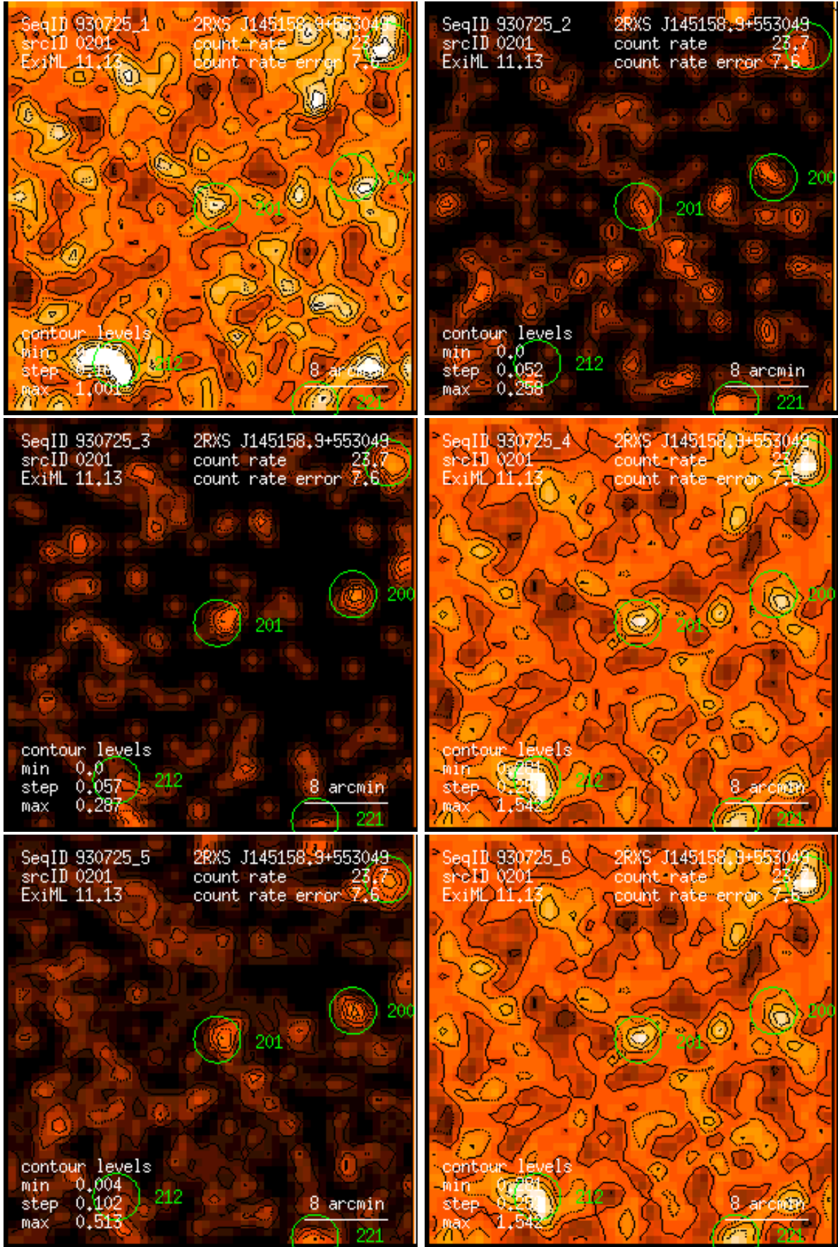
Figure 201: RASS 930725: detection 0201: band rate images, Gaussian filter: (1) PSPC channels 11 – 41, (2) 52 – 90, (3) 91 – 201, (4) 11 – 235, (5) 52 – 201, (6) 11 – 201. Broad band rates in counts/ks. Band rate contour levels in counts/ks/arcmin 2 .
