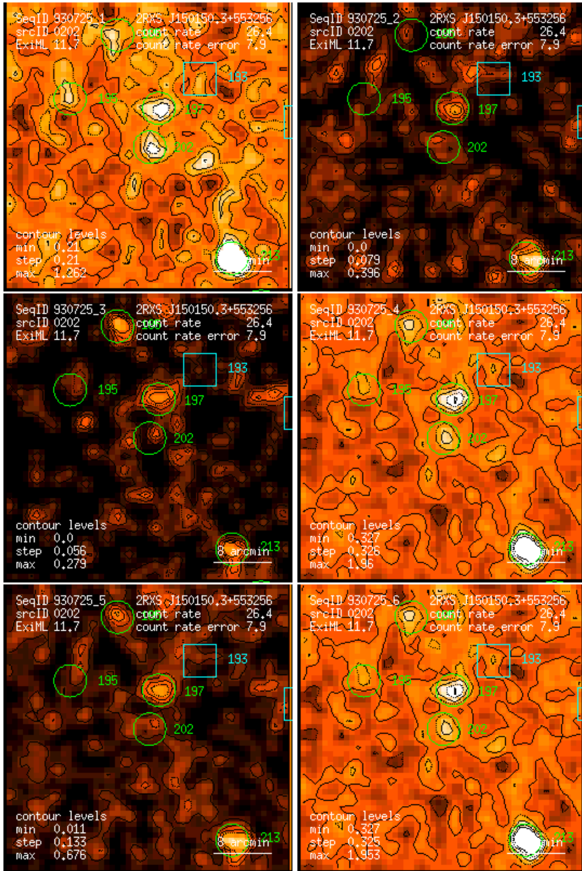
Figure 202: RASS 930725: detection 0202: band rate images, Gaussian filter: (1) PSPC channels 11 – 41, (2) 52 – 90, (3) 91 – 201, (4) 11 – 235, (5) 52 – 201, (6) 11 – 201. Broad band rates in counts/ks. Band rate contour levels in counts/ks/arcmin 2 .
