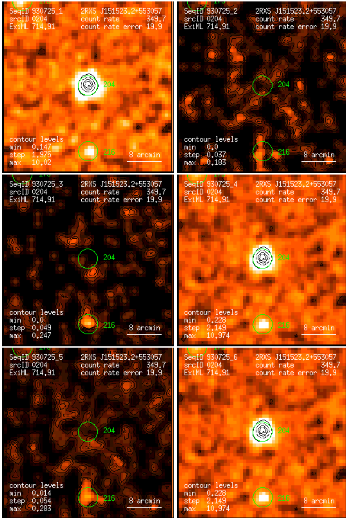
Figure 204: RASS 930725: detection 0204: band rate images, Gaussian filter: (1) PSPC channels 11 – 41, (2) 52 – 90, (3) 91 – 201, (4) 11 – 235, (5) 52 – 201, (6) 11 – 201. Broad band rates in counts/ks. Band rate contour levels in counts/ks/arcmin 2 .
