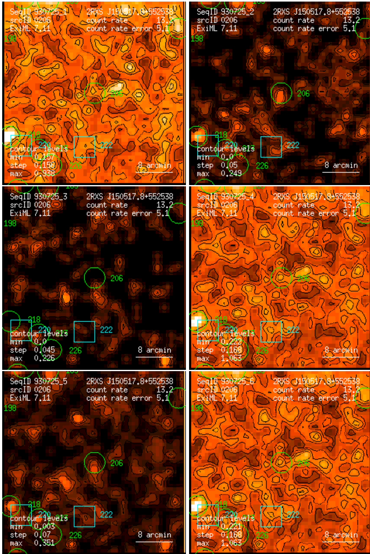
Figure 206: RASS 930725: detection 0206: band rate images, Gaussian filter: (1) PSPC channels 11 – 41, (2) 52 – 90, (3) 91 – 201, (4) 11 – 235, (5) 52 – 201, (6) 11 – 201. Broad band rates in counts/ks. Band rate contour levels in counts/ks/arcmin 2 .
