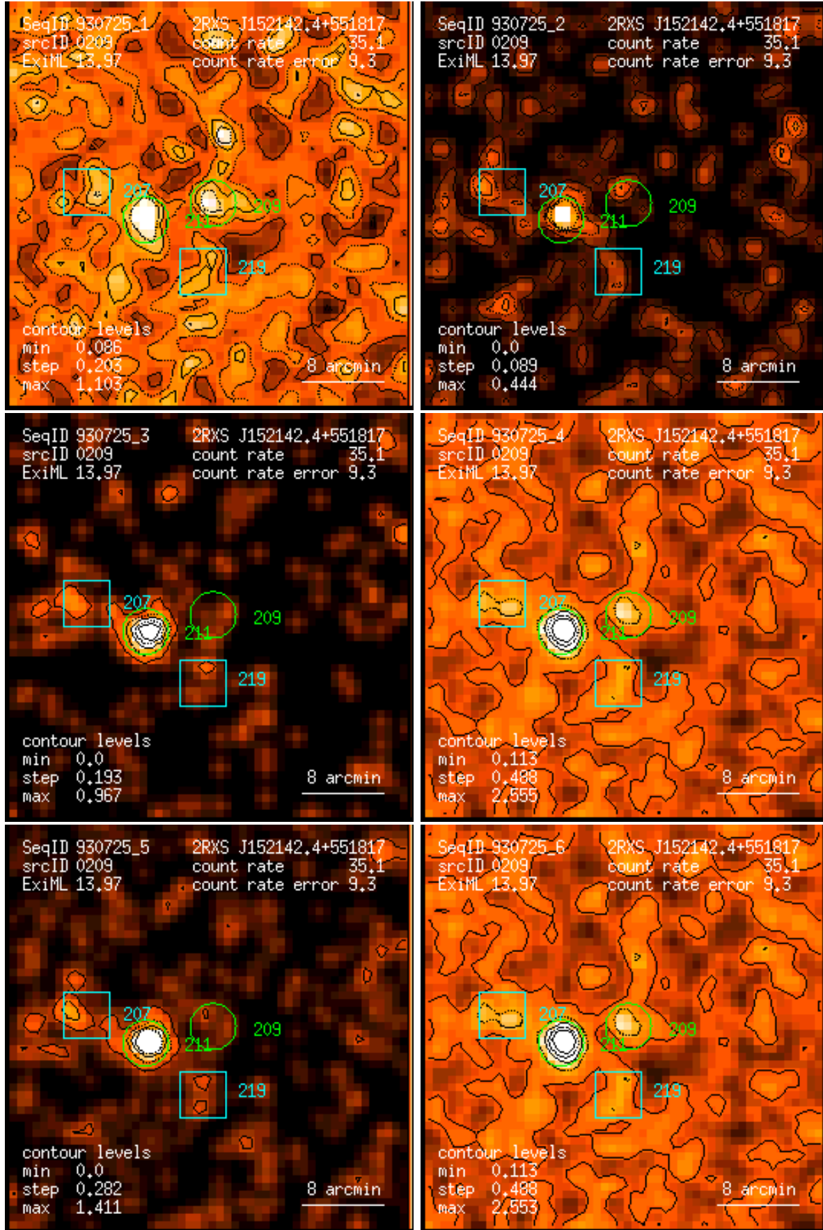
Figure 209: RASS 930725: detection 0209: band rate images, Gaussian filter: (1) PSPC channels 11 – 41, (2) 52 – 90, (3) 91 – 201, (4) 11 – 235, (5) 52 – 201, (6) 11 – 201. Broad band rates in counts/ks. Band rate contour levels in counts/ks/arcmin 2 .
