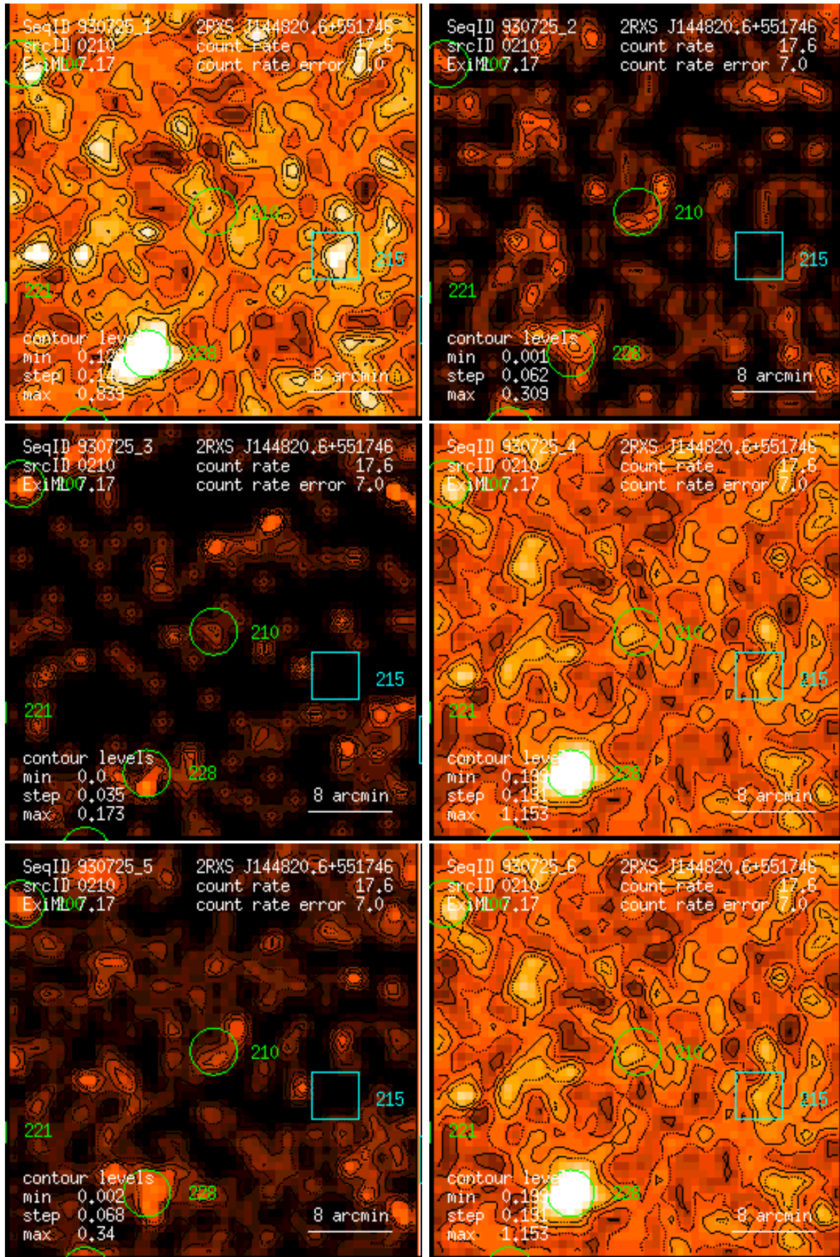
Figure 210: RASS 930725: detection 0210: band rate images, Gaussian filter: (1) PSPC channels 11 – 41, (2) 52 – 90, (3) 91 – 201, (4) 11 – 235, (5) 52 – 201, (6) 11 – 201. Broad band rates in counts/ks. Band rate contour levels in counts/ks/arcmin 2 .
