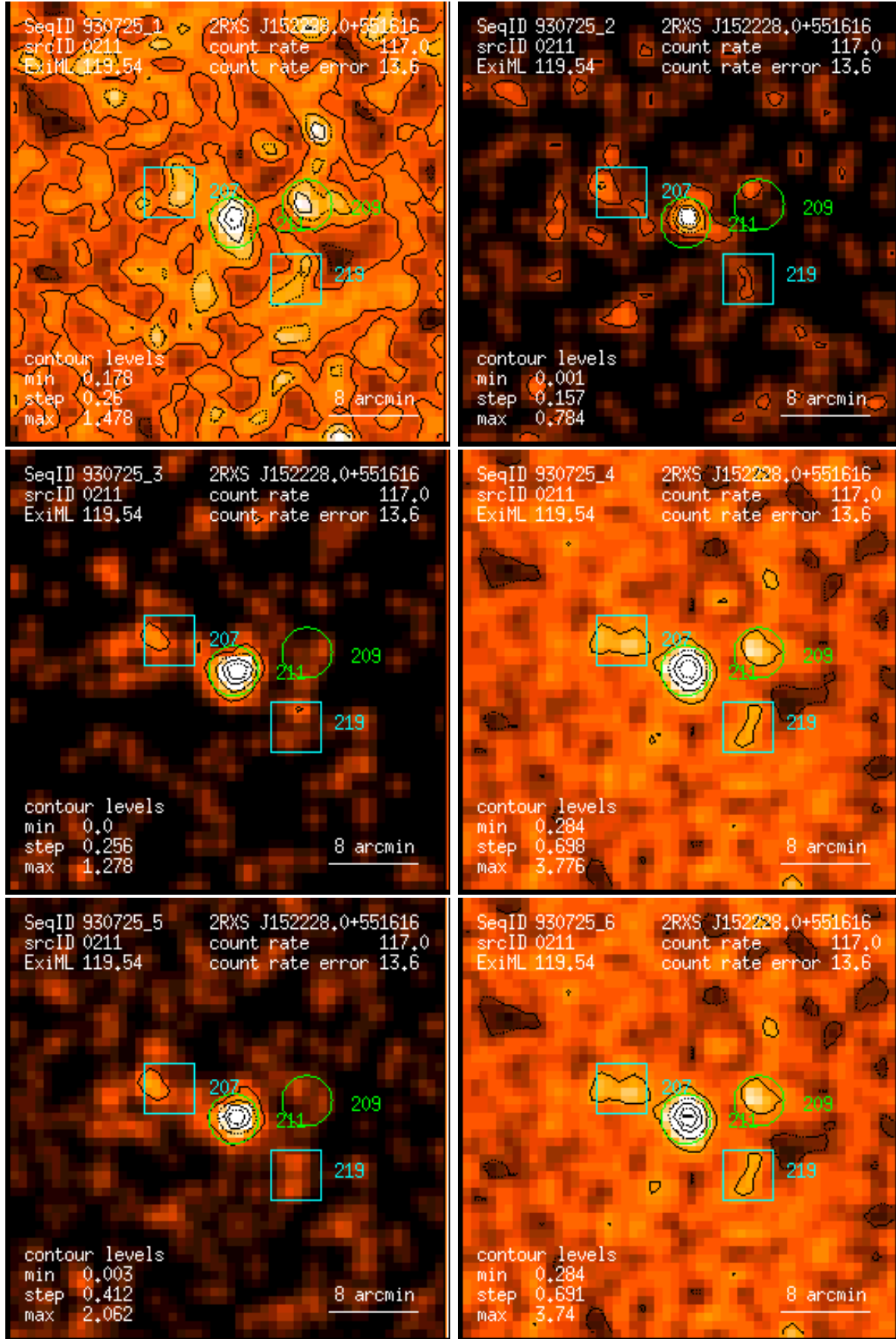
Figure 211: RASS 930725: detection 0211: band rate images, Gaussian filter: (1) PSPC channels 11 – 41, (2) 52 – 90, (3) 91 – 201, (4) 11 – 235, (5) 52 – 201, (6) 11 – 201. Broad band rates in counts/ks. Band rate contour levels in counts/ks/arcmin 2 .
