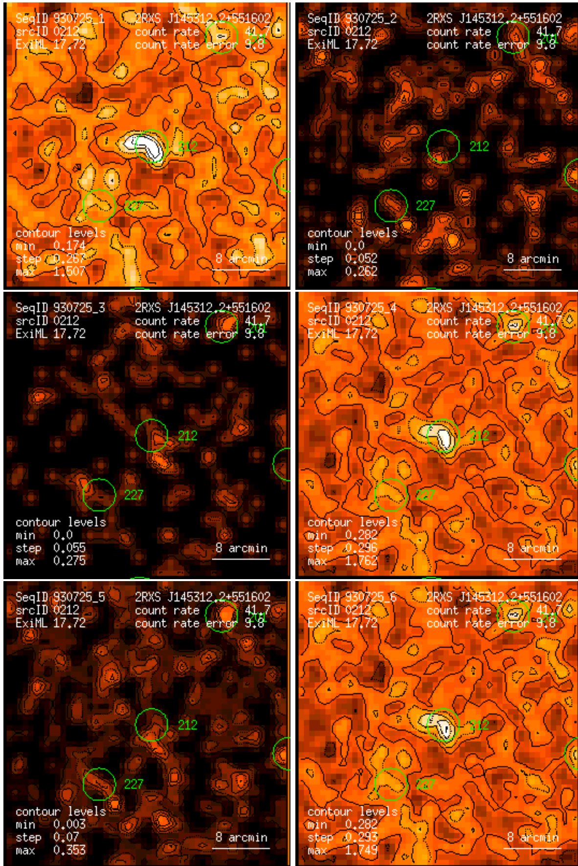
Figure 212: RASS 930725: detection 0212: band rate images, Gaussian filter: (1) PSPC channels 11 – 41, (2) 52 – 90, (3) 91 – 201, (4) 11 – 235, (5) 52 – 201, (6) 11 – 201. Broad band rates in counts/ks. Band rate contour levels in counts/ks/arcmin 2 .
