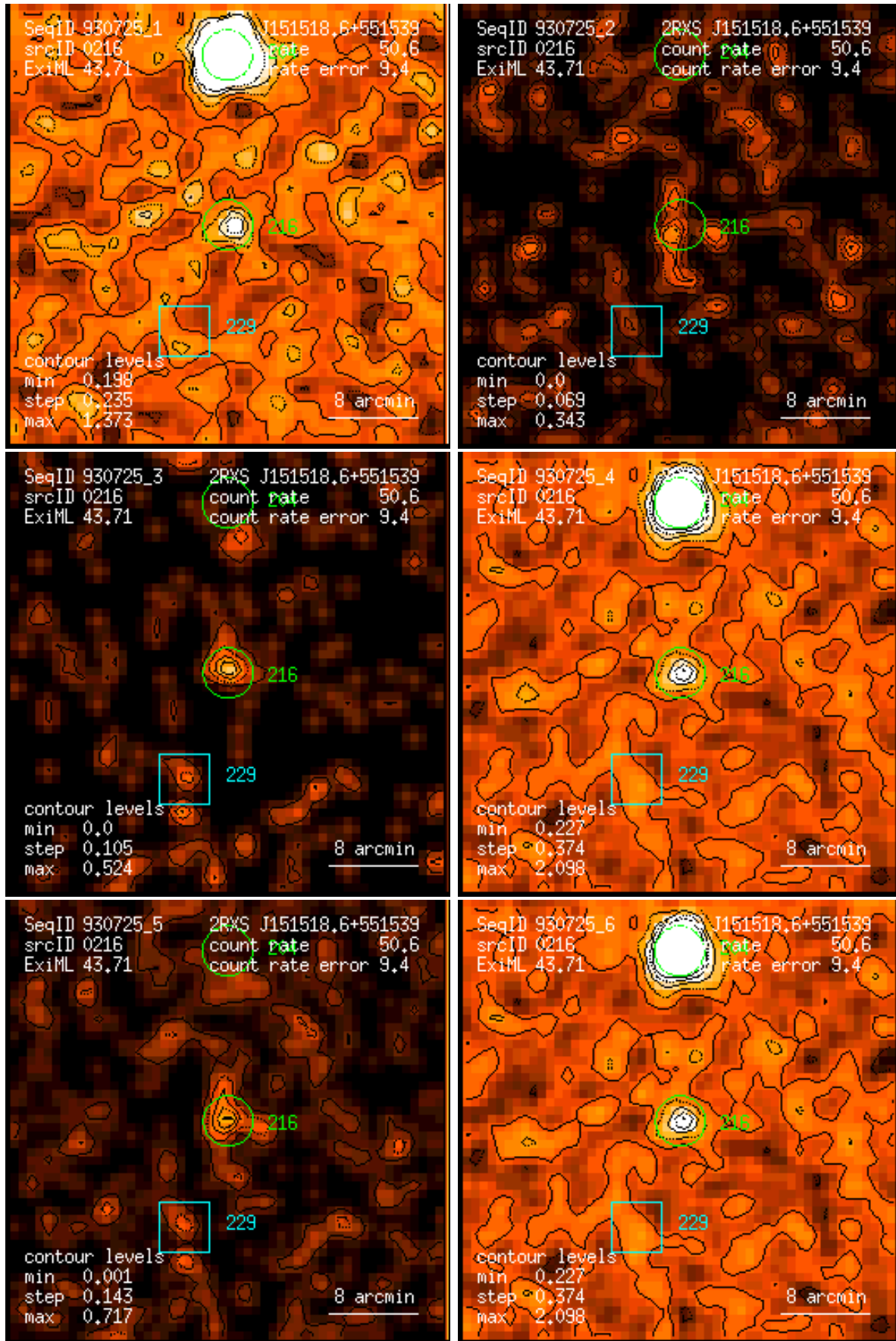
Figure 216: RASS 930725: detection 0216: band rate images, Gaussian filter: (1) PSPC channels 11 – 41, (2) 52 – 90, (3) 91 – 201, (4) 11 – 235, (5) 52 – 201, (6) 11 – 201. Broad band rates in counts/ks. Band rate contour levels in counts/ks/arcmin 2 .
