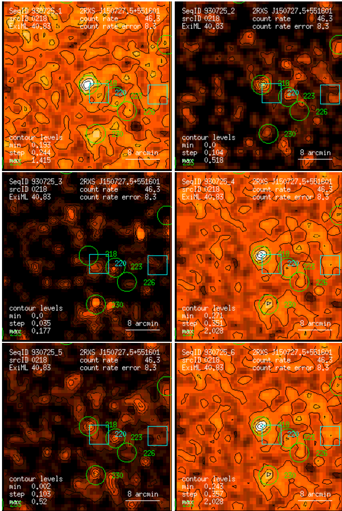
Figure 218: RASS 930725: detection 0218: band rate images, Gaussian filter: (1) PSPC channels 11 – 41, (2) 52 – 90, (3) 91 – 201, (4) 11 – 235, (5) 52 – 201, (6) 11 – 201. Broad band rates in counts/ks. Band rate contour levels in counts/ks/arcmin 2 .
