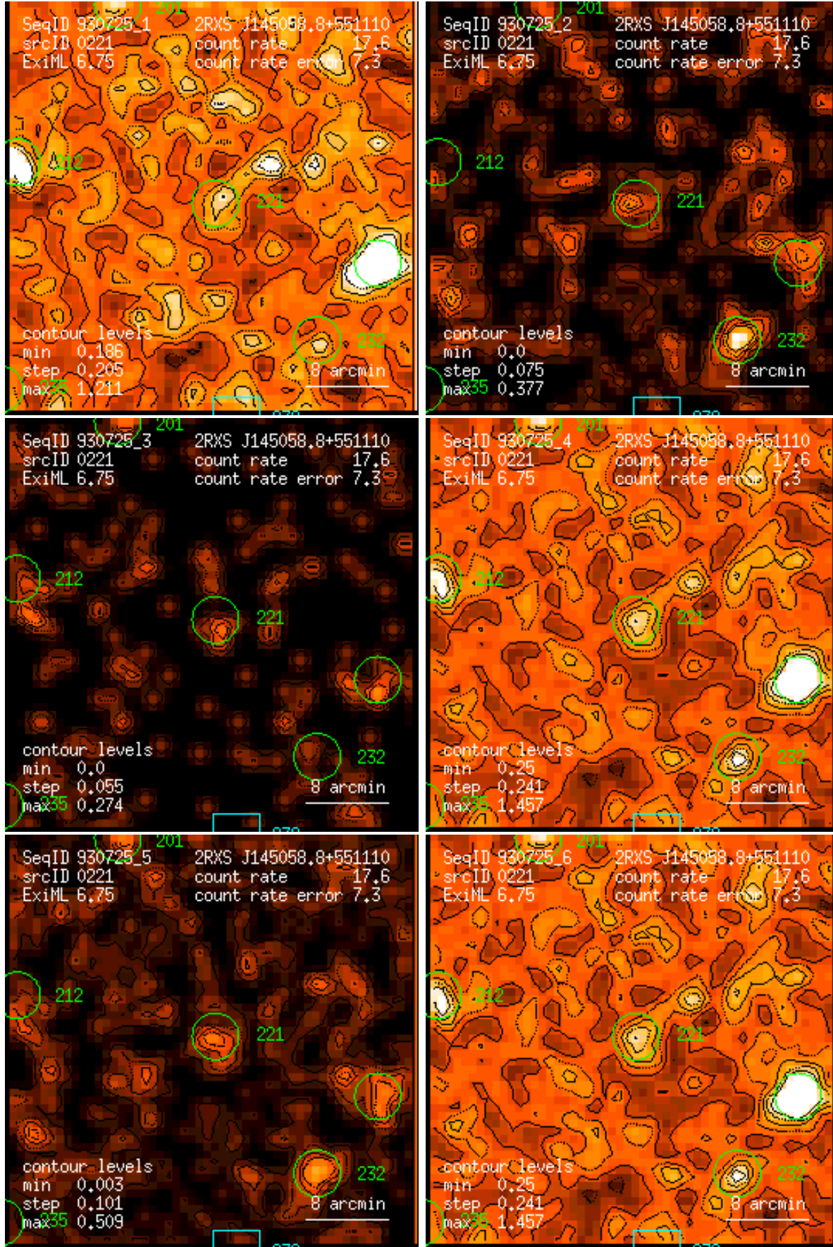
Figure 221: RASS 930725: detection 0221: band rate images, Gaussian filter: (1) PSPC channels 11 – 41, (2) 52 – 90, (3) 91 – 201, (4) 11 – 235, (5) 52 – 201, (6) 11 – 201. Broad band rates in counts/ks. Band rate contour levels in counts/ks/arcmin 2 .
