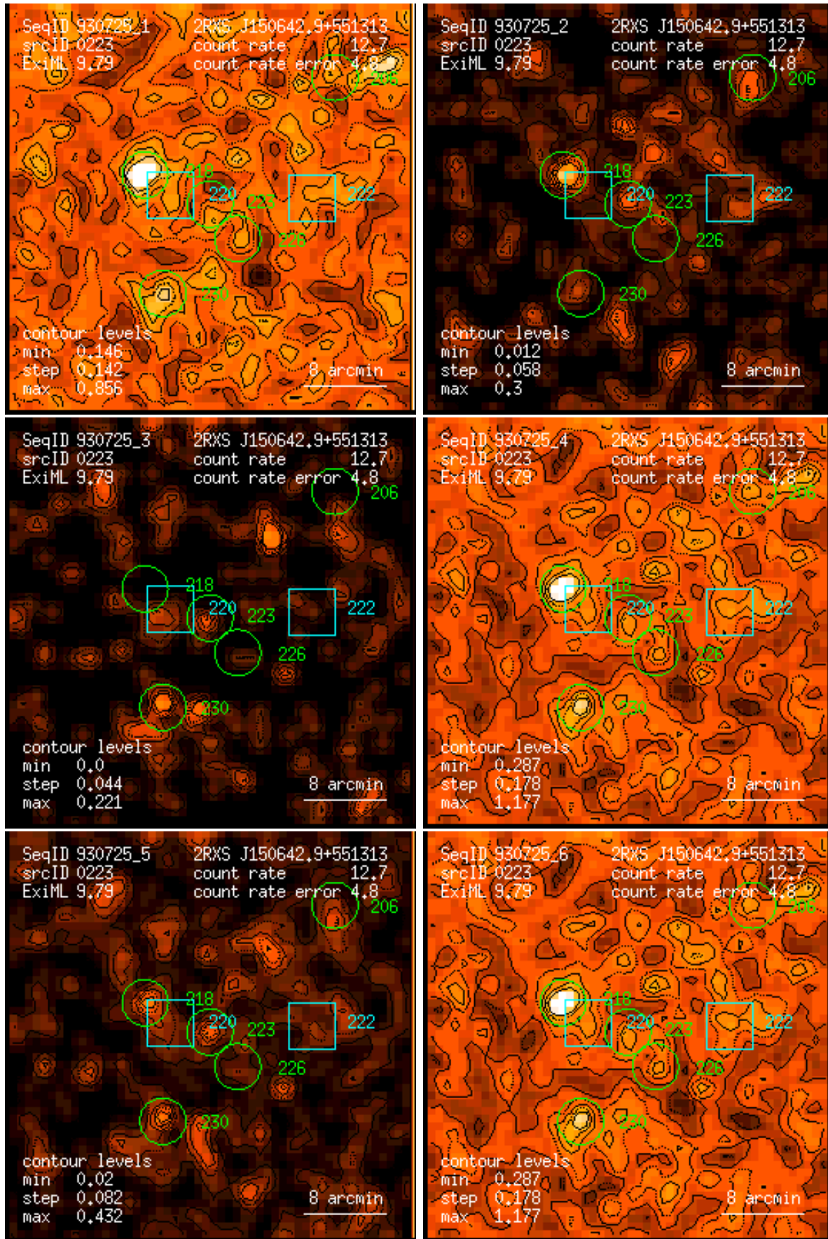
Figure 223: RASS 930725: detection 0223: band rate images, Gaussian filter: (1) PSPC channels 11 – 41, (2) 52 – 90, (3) 91 – 201, (4) 11 – 235, (5) 52 – 201, (6) 11 – 201. Broad band rates in counts/ks. Band rate contour levels in counts/ks/arcmin 2 .
