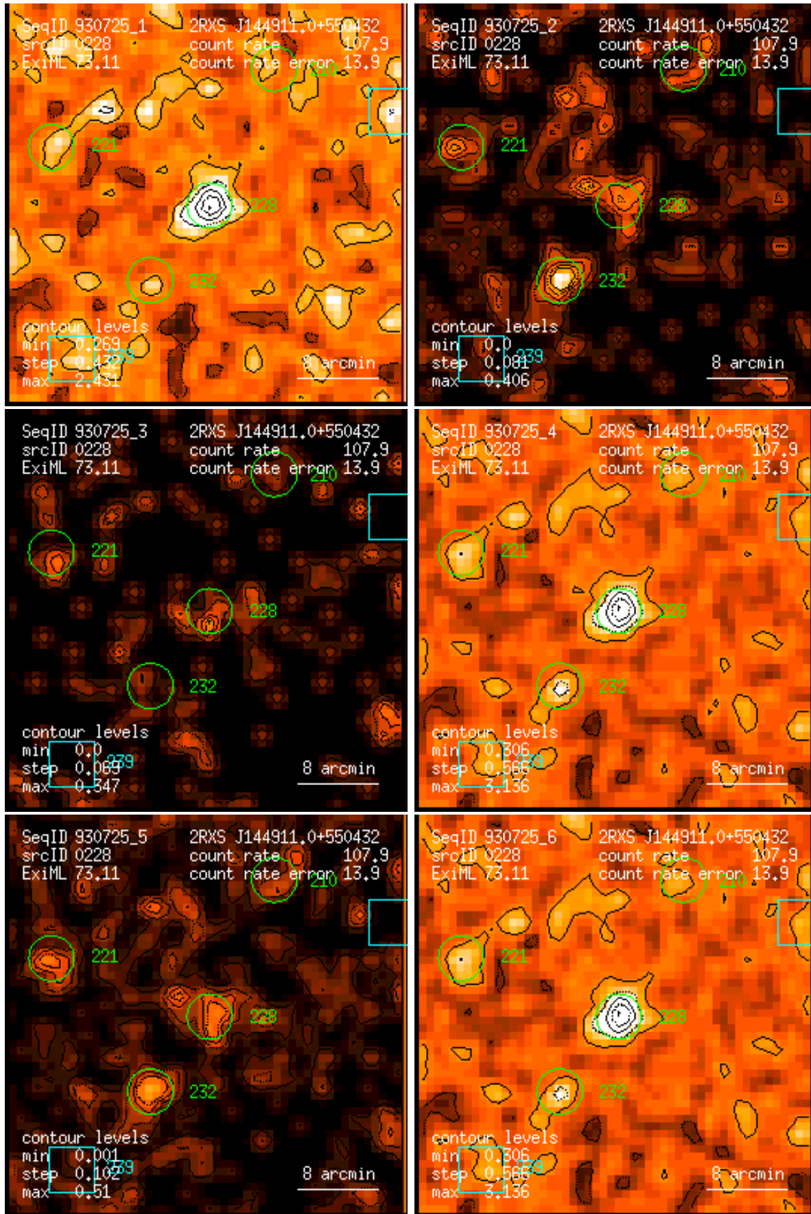
Figure 228: RASS 930725: detection 0228: band rate images, Gaussian filter: (1) PSPC channels 11 – 41, (2) 52 – 90, (3) 91 – 201, (4) 11 – 235, (5) 52 – 201, (6) 11 – 201. Broad band rates in counts/ks. Band rate contour levels in counts/ks/arcmin 2 .
