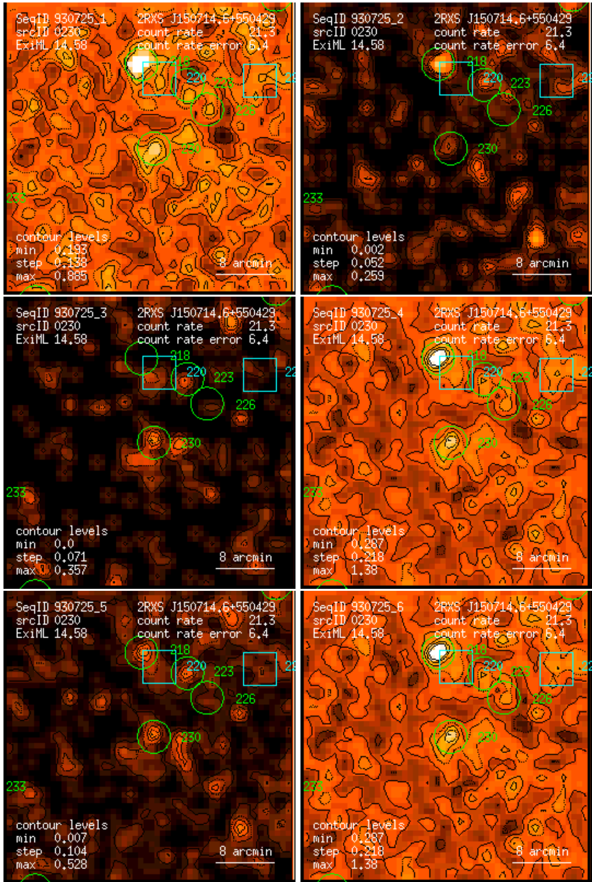
Figure 230: RASS 930725: detection 0230: band rate images, Gaussian filter: (1) PSPC channels 11 – 41, (2) 52 – 90, (3) 91 – 201, (4) 11 – 235, (5) 52 – 201, (6) 11 – 201. Broad band rates in counts/ks. Band rate contour levels in counts/ks/arcmin 2 .
