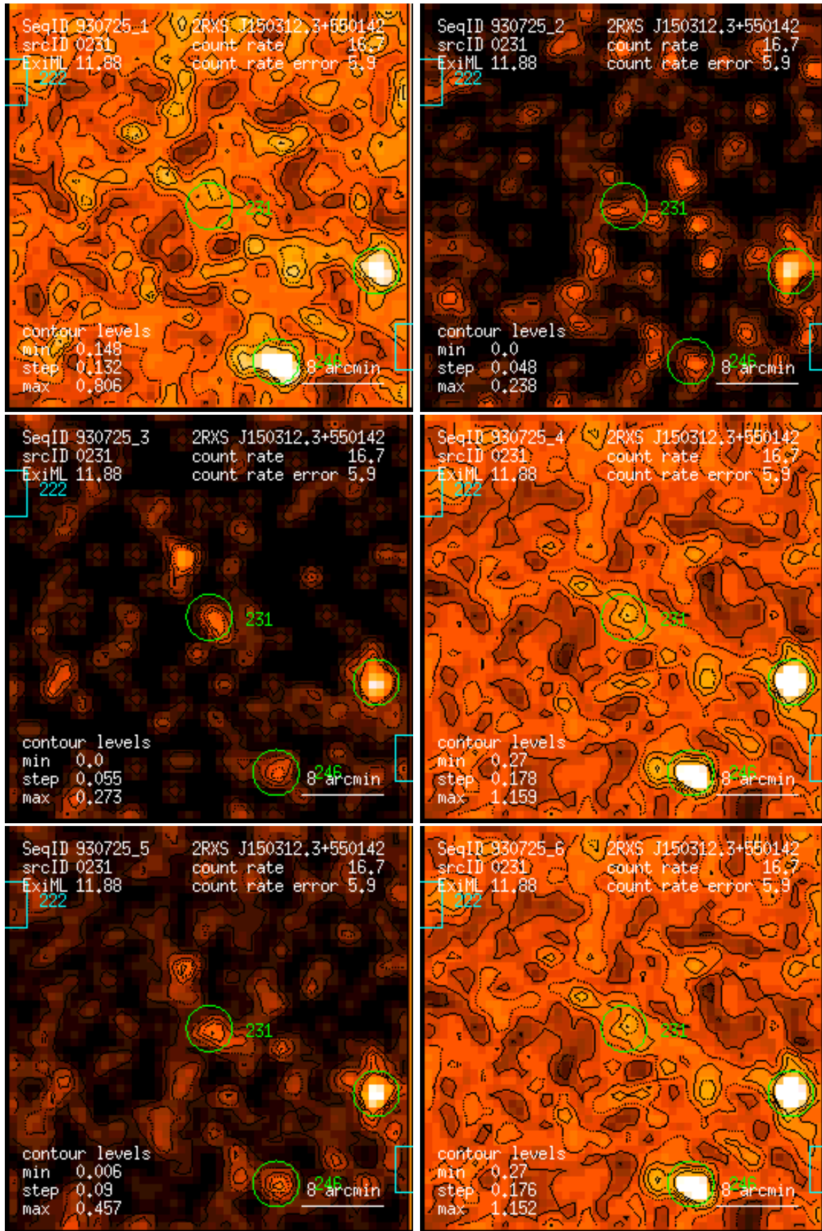
Figure 231: RASS 930725: detection 0231: band rate images, Gaussian filter: (1) PSPC channels 11 – 41, (2) 52 – 90, (3) 91 – 201, (4) 11 – 235, (5) 52 – 201, (6) 11 – 201. Broad band rates in counts/ks. Band rate contour levels in counts/ks/arcmin 2 .
