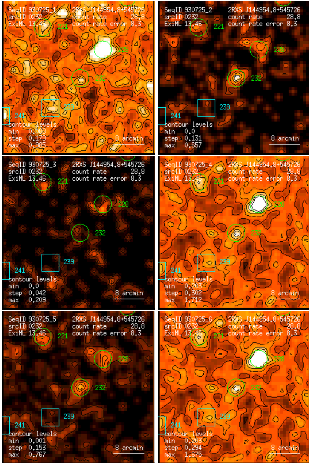
Figure 232: RASS 930725: detection 0232: band rate images, Gaussian filter: (1) PSPC channels 11 – 41, (2) 52 – 90, (3) 91 – 201, (4) 11 – 235, (5) 52 – 201, (6) 11 – 201. Broad band rates in counts/ks. Band rate contour levels in counts/ks/arcmin 2 .
