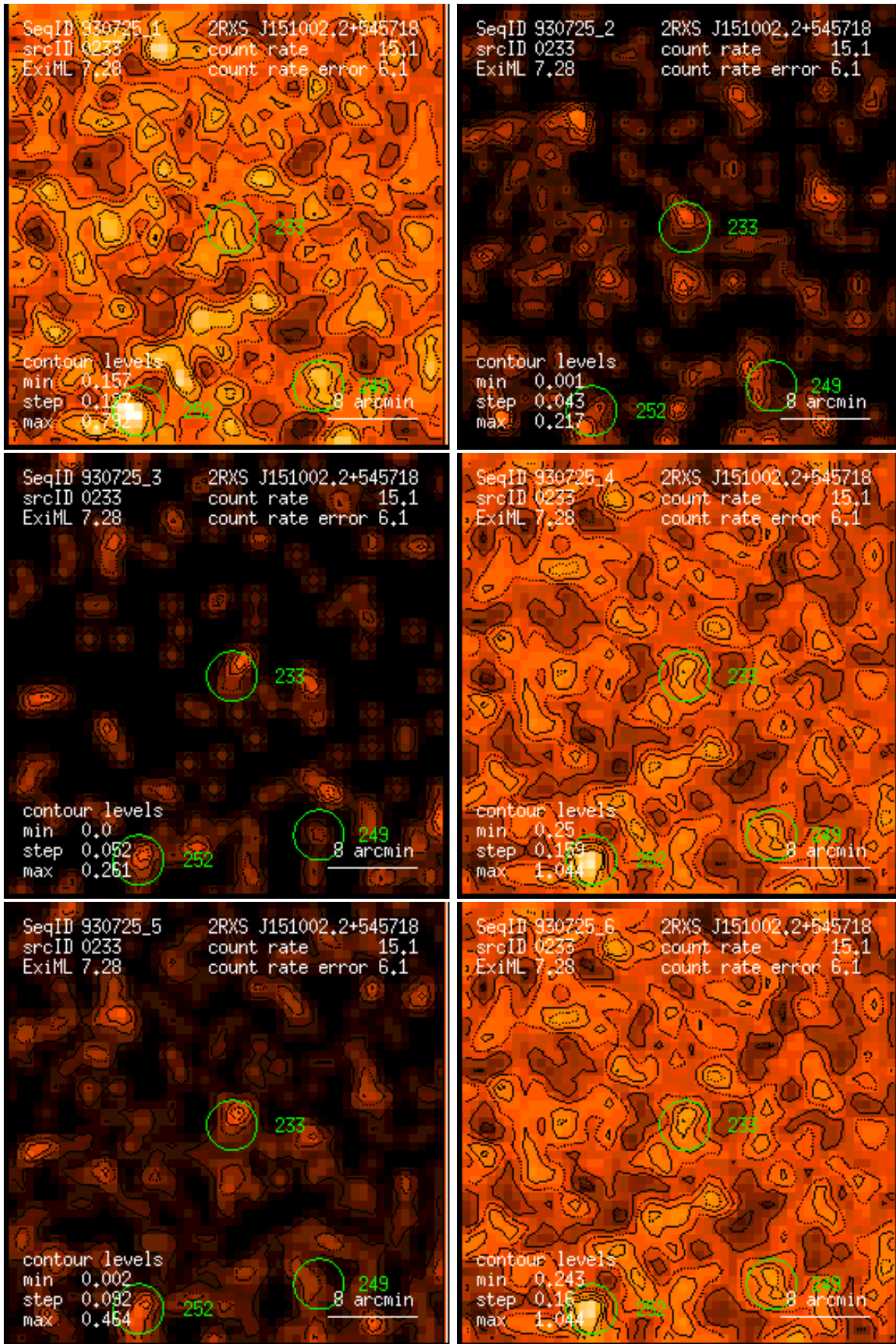
Figure 233: RASS 930725: detection 0233: band rate images, Gaussian filter: (1) PSPC channels 11 – 41, (2) 52 – 90, (3) 91 – 201, (4) 11 – 235, (5) 52 – 201, (6) 11 – 201. Broad band rates in counts/ks. Band rate contour levels in counts/ks/arcmin 2 .
